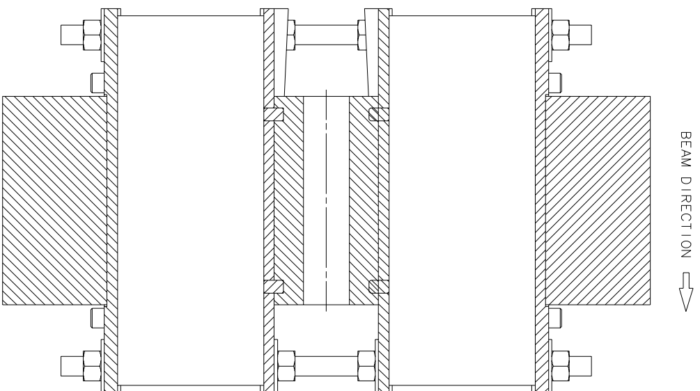
SECTION B-B
