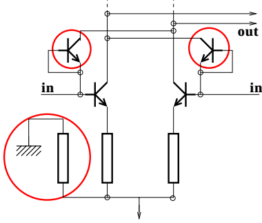
Figure 12: multiplexer detail
