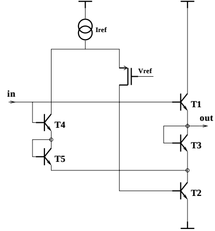
Figure 13: buffer design
