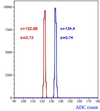
Figure 16: noise
