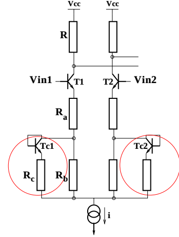
Figure 4: parallel compensation
