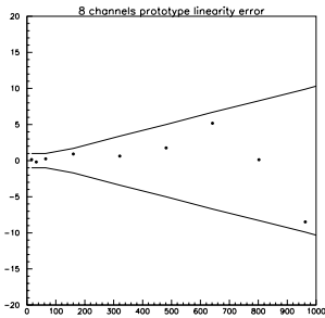
Figure 14: linearity
