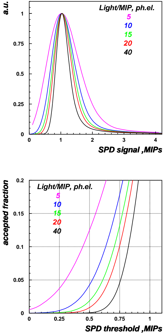
Figure 15: The effect of light photo-statistical fluctuations on the MIP registration in SPD is shown. On the upper plot one can see the distortion of SPD spectrum in case of 5, 10, 15, 20 and 40 ph.el. collected per MIP . The MIP registration inefficiency as function of applied threshold is demonstrated on the bottom plot.
