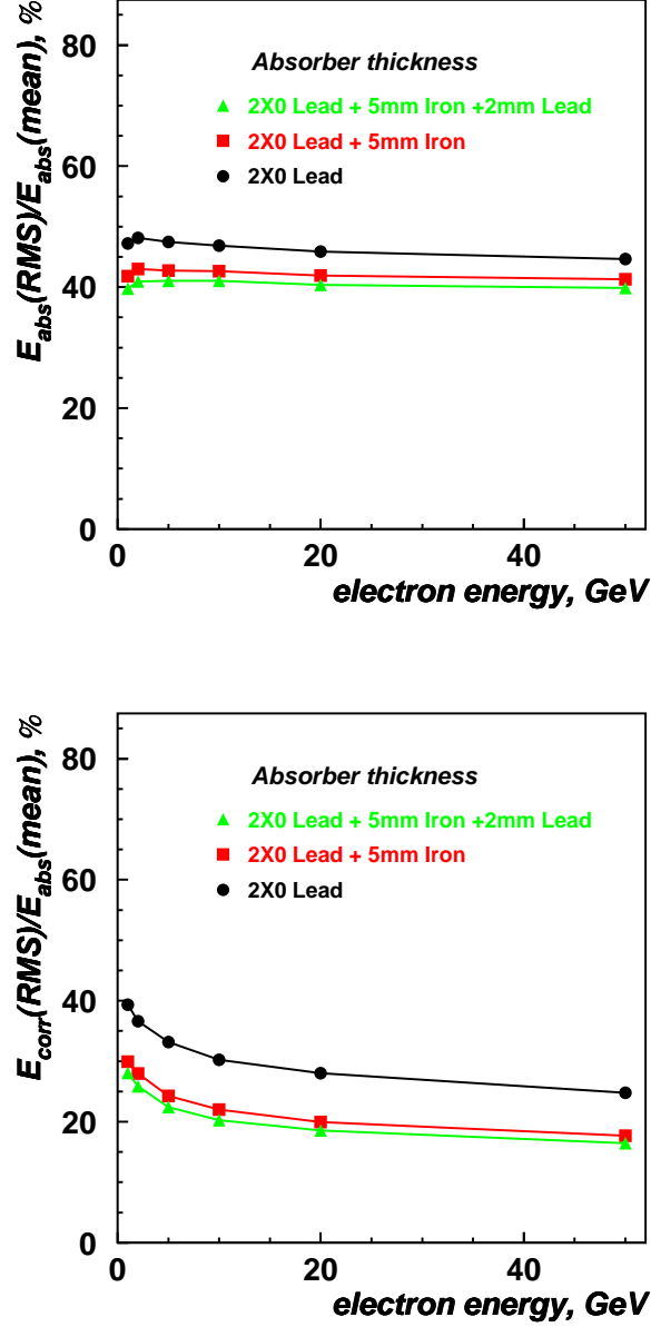
Figure 12: Ratio of the fluctuations (r.m.s.) of the energy lost in the lead absorber and in the passive material of ECAL to its mean value is plotted vs beam energy on the top figure. The same data after the correction with PS signal are shown on the bottom plot. From comparison with fig. 9 one can see that the correction works better for the front material of ECAL then for an additional absorber of PS.
