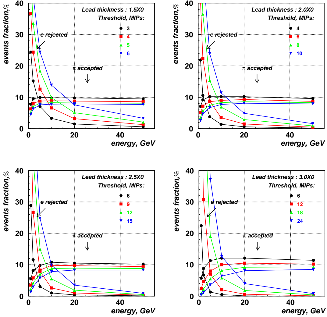
Figure 4: \pi/e rejection in PS for constant value of the threshold. To obtain both good pion rejection and high electron acceptance over all energy scale, one has to vary the threshold value with the beam energy.
