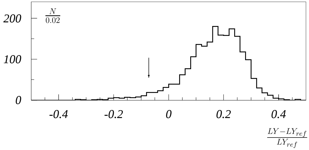
Figure 7: Results of the "hedgehog" test as measures for groups of three tiles. Shown is the light yield relative to that of a reference tile. The r.m.s. for the tiles used for module assembly ( LY > 0.93 \cdot LY_{ref} , corresponding region is to the right from arrow ) is \approx 0.09 . For details see the text
