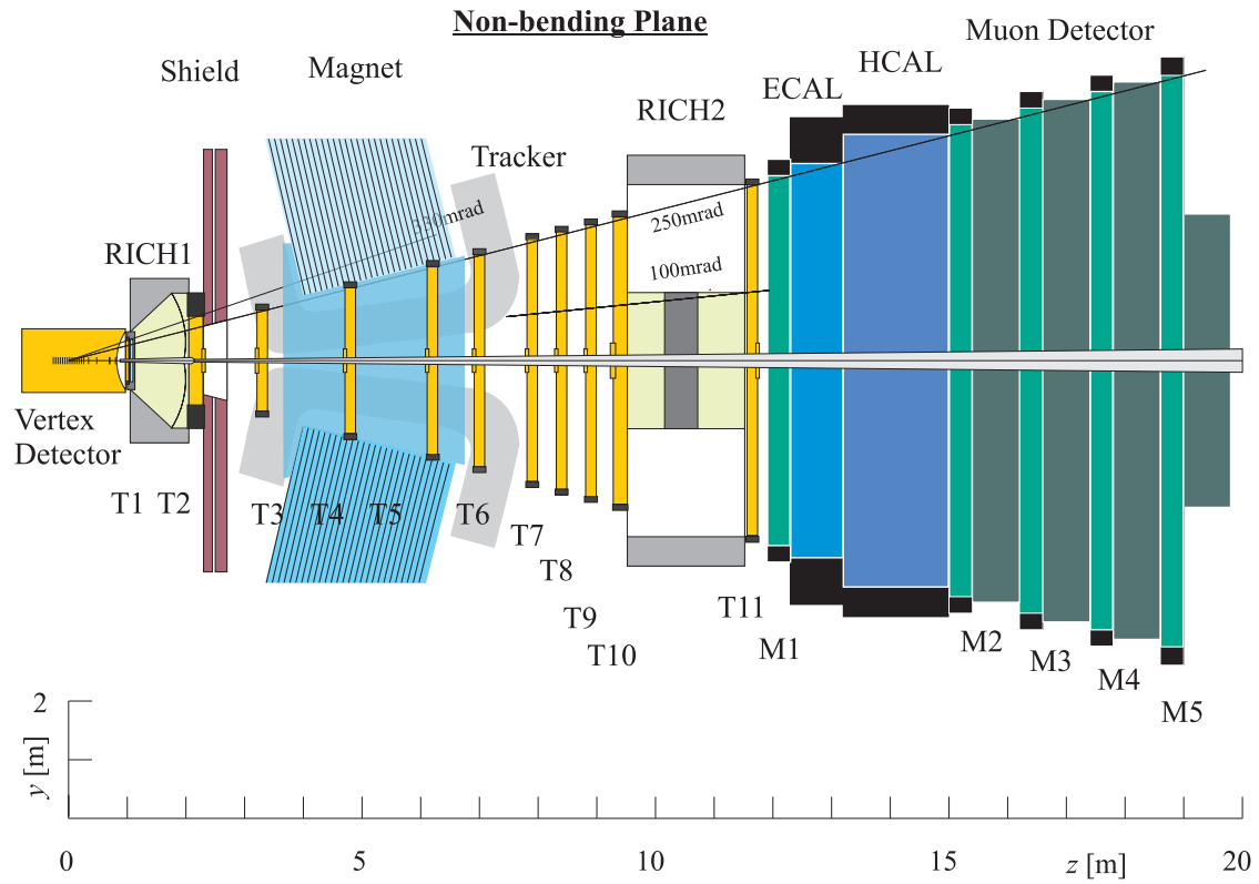
Figure 2: LHCb detector
