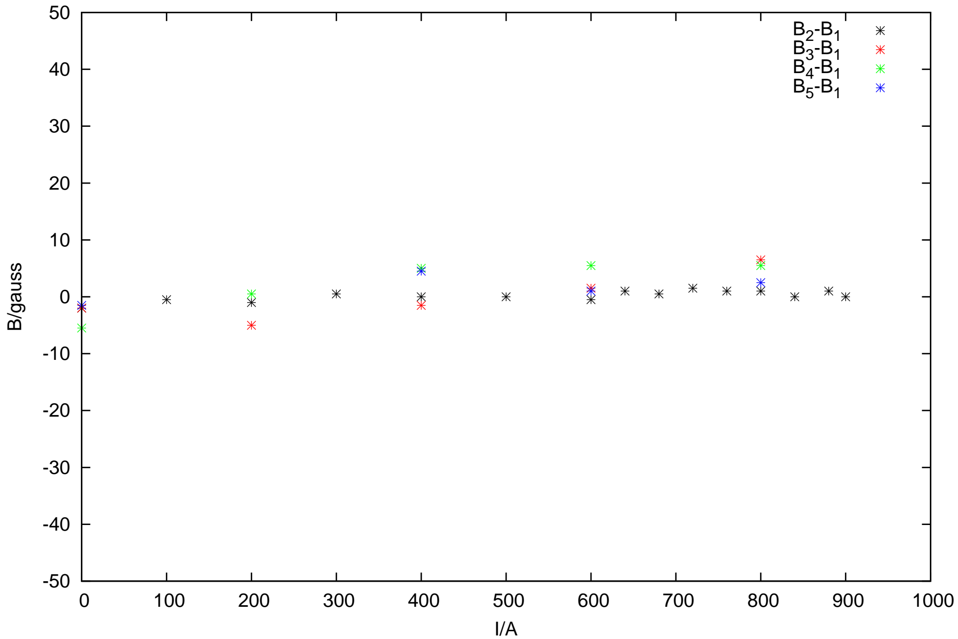
\Delta B vs I, B_i - B_1 , probe s1
