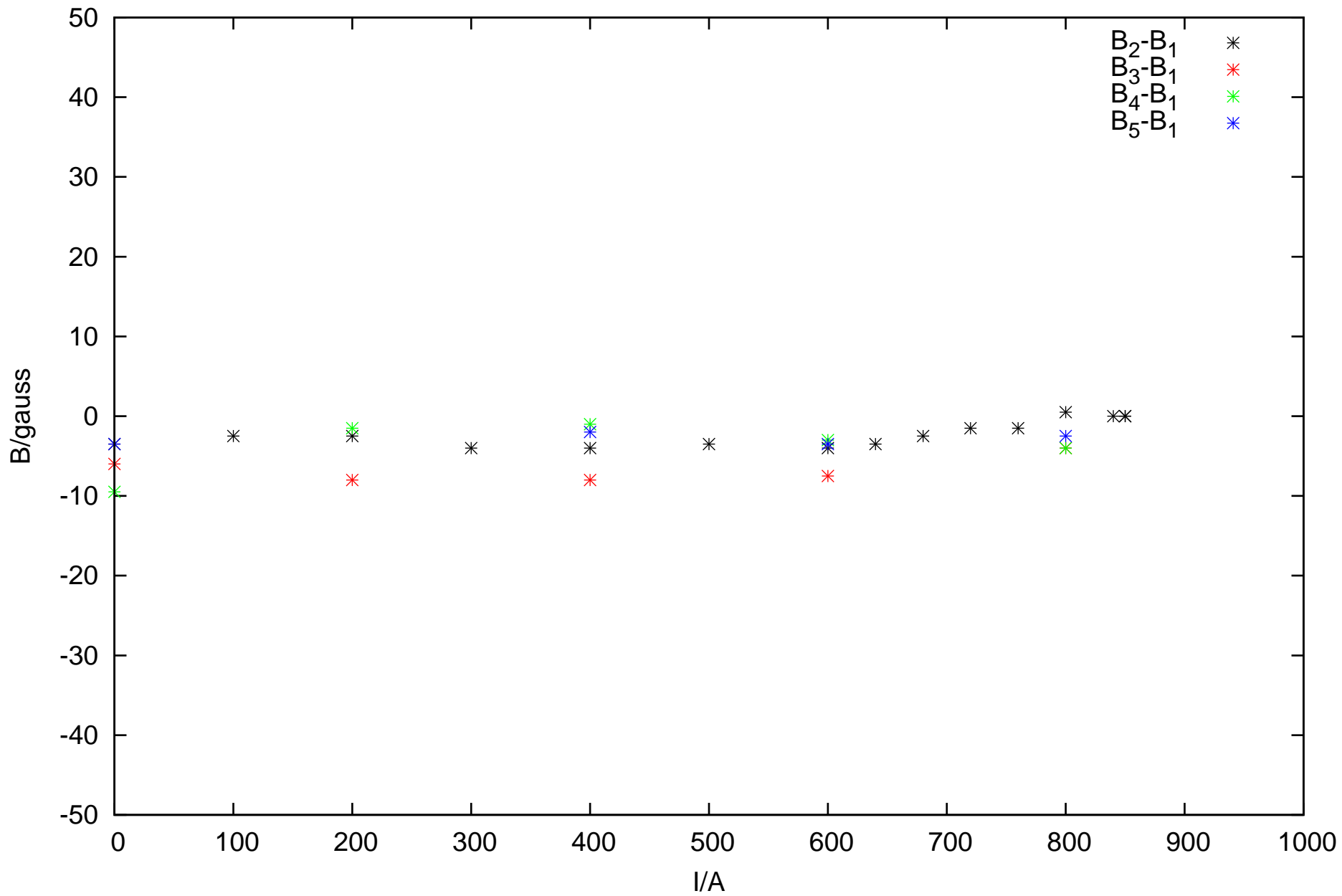
\Delta B vs I, B_i - B_1 , probe s2
