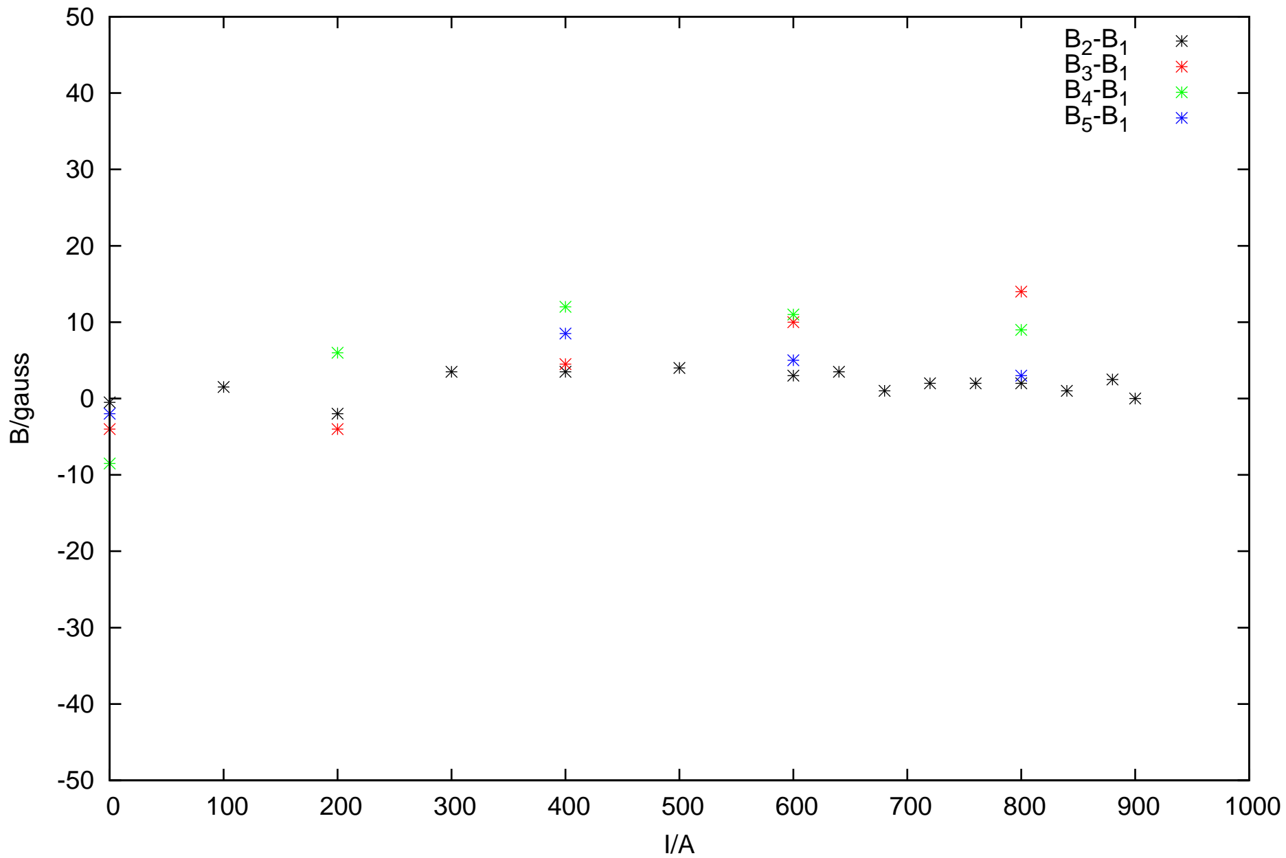
\Delta B vs I, B_i - B_1 , probe bb
