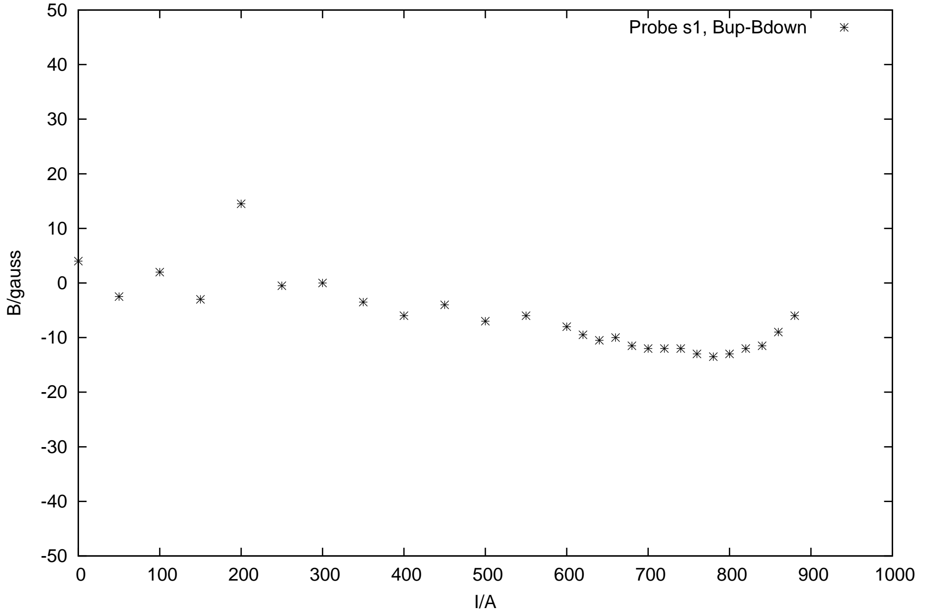
\Delta B vs I, Bup-Bdown, iter1, probe s1
