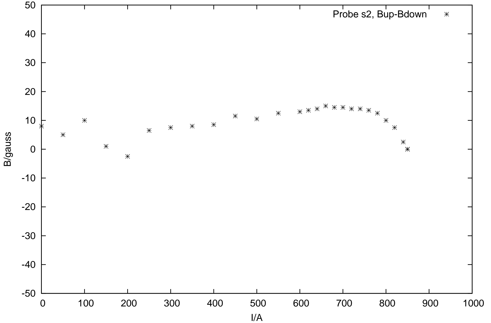
\Delta B vs I, Bup-Bdown, iter1, probe s2
