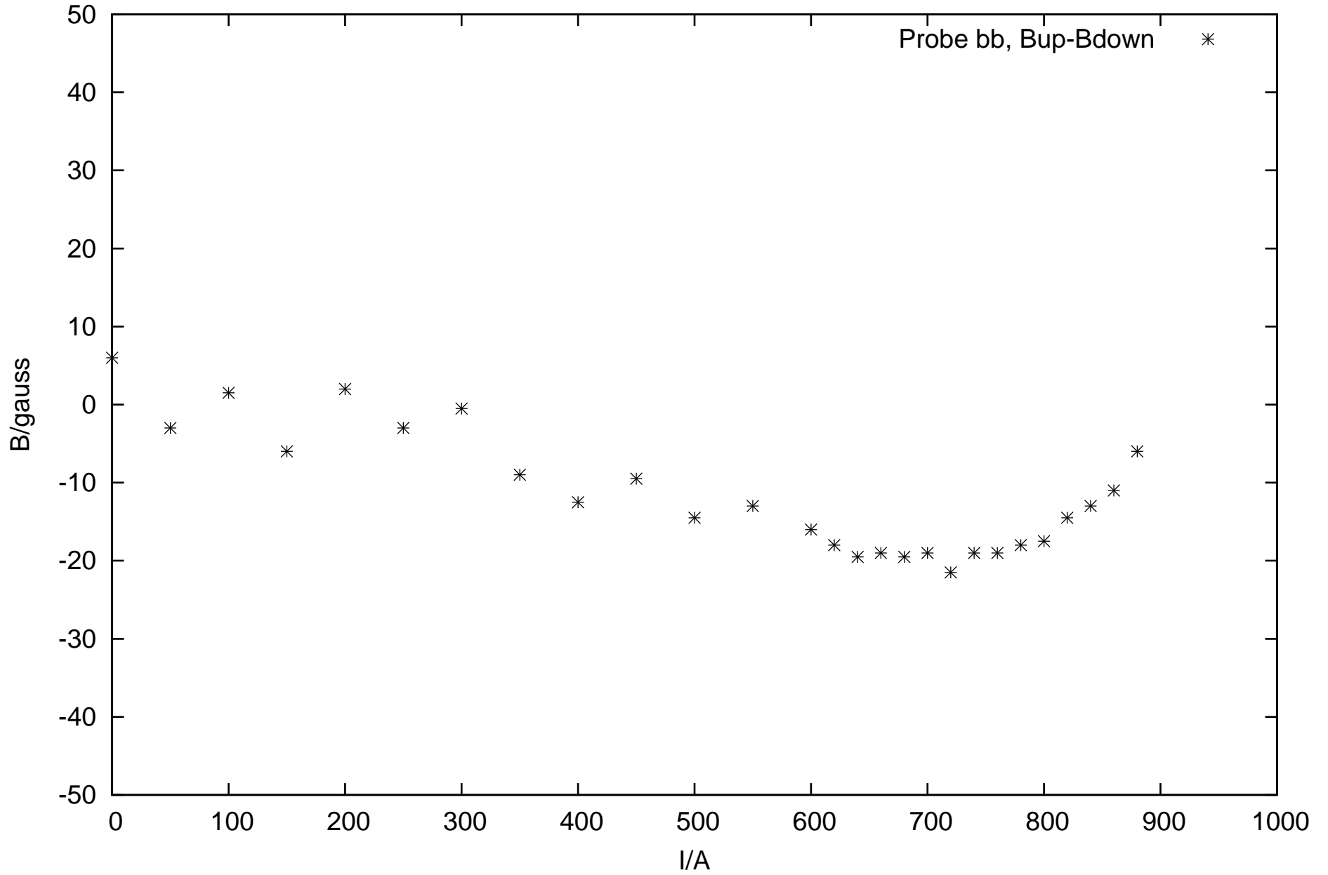
\Delta B vs I, Bup-Bdown, iter1, probe bb
