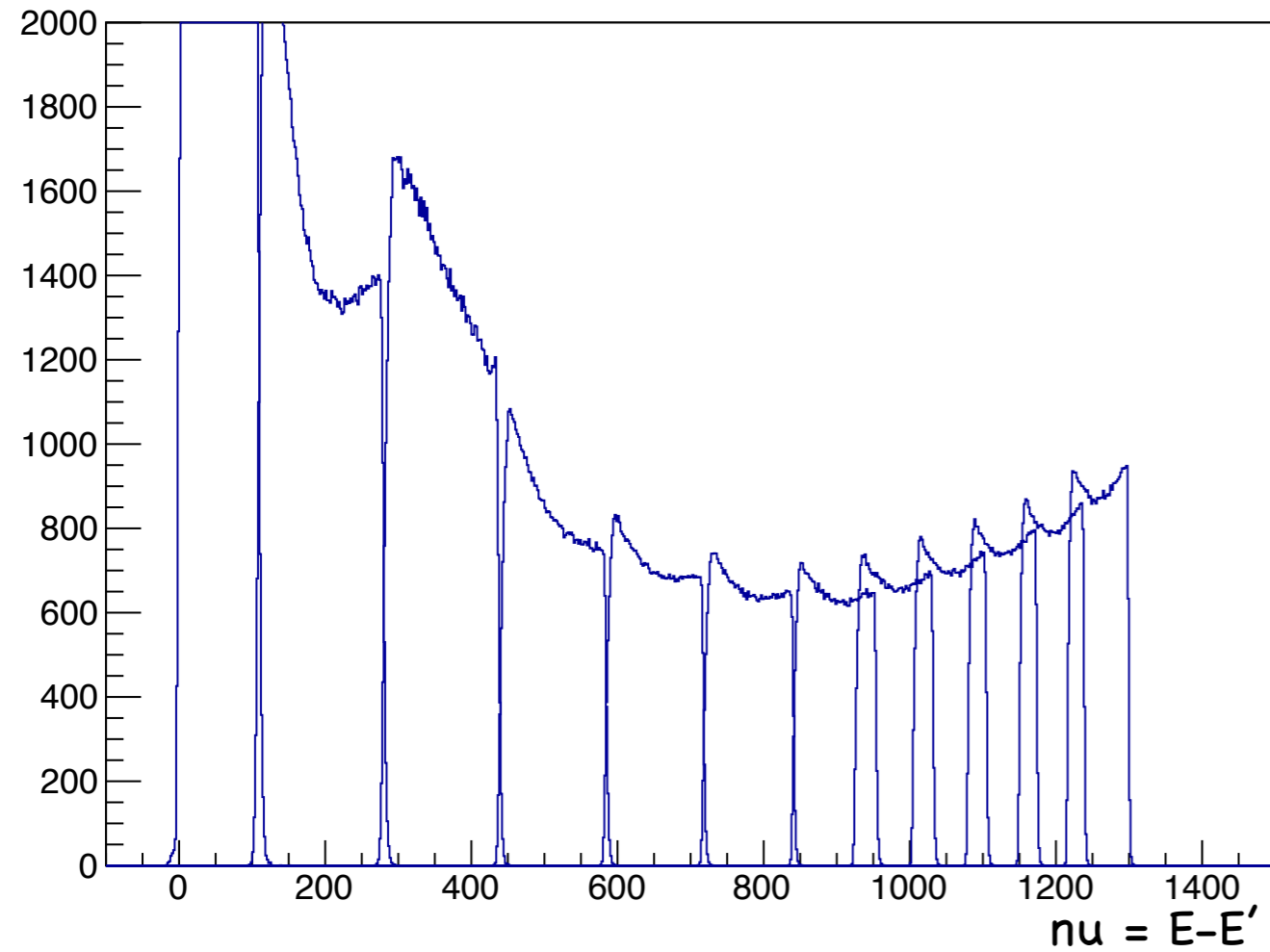
2.2 GeV longitudinal, effective yield
