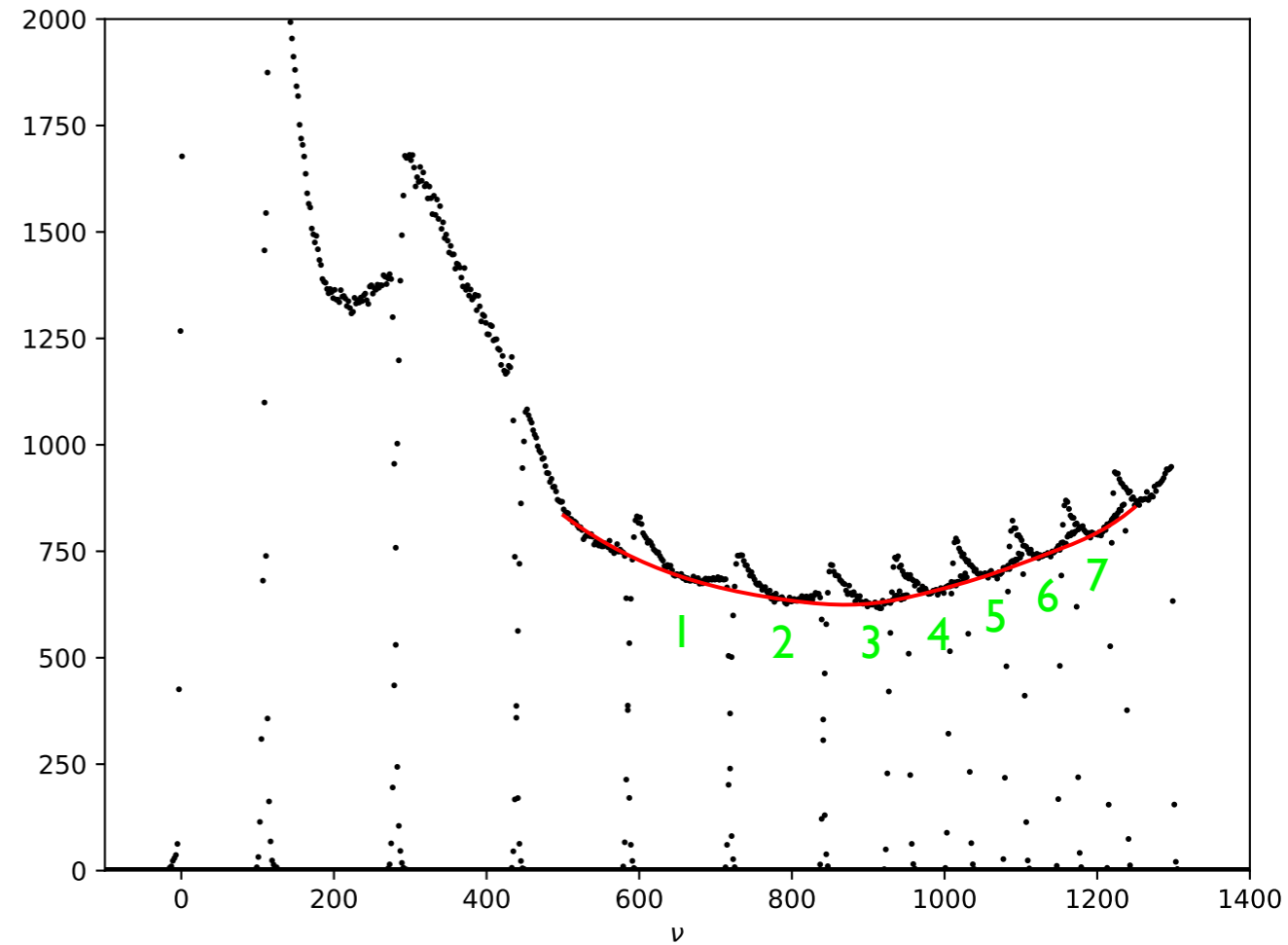
Fit the correction with 7 momentum settings
