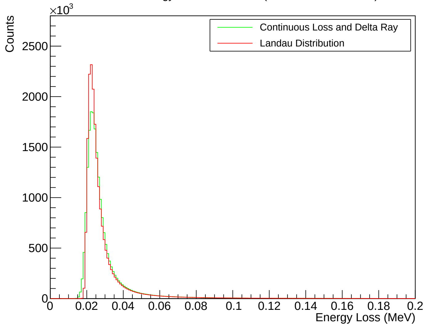
Ionization Energy Loss Distribution ( ^{12}\text{C} Thickness 0.1mm)
