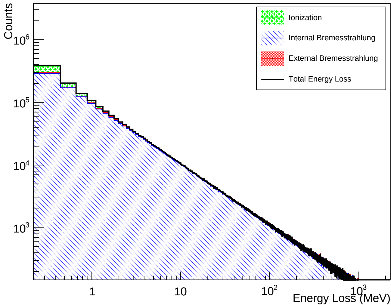
Ionization Energy Loss Distribution ( ^{12}\text{C} Thickness 0.1mm)
