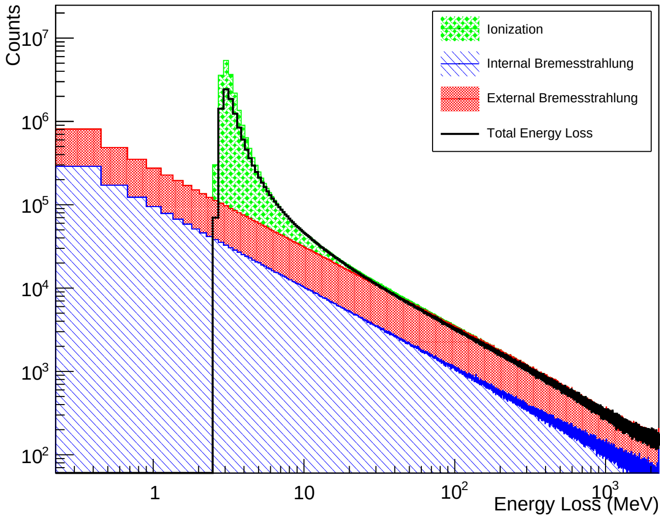
Ionization Energy Loss Distribution ( ^{12}\text{C} Thickness 10.0mm)
