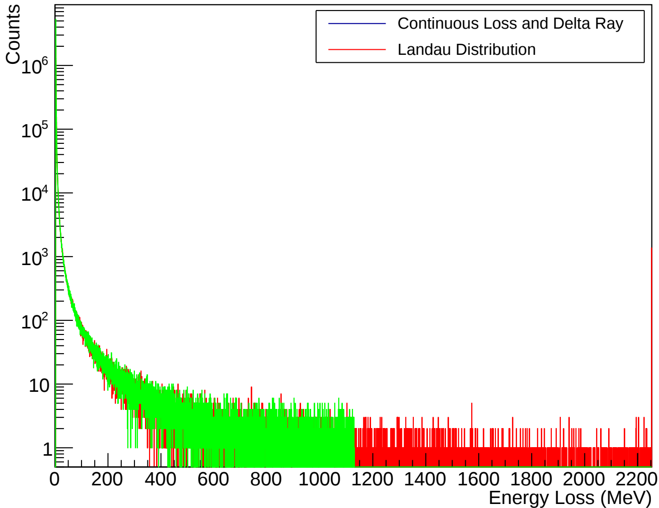
Ionization Energy Distribution ( ^{12}\text{C} Thickness 10.0mm)
