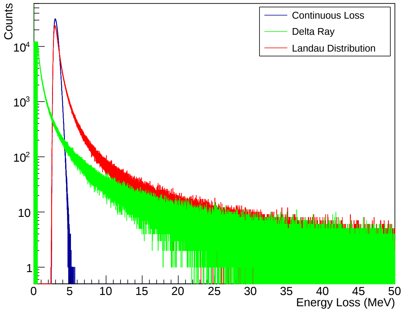
Ionization Energy Loss Distribution ( ^{12}\text{C} Thickness 10.0mm)
