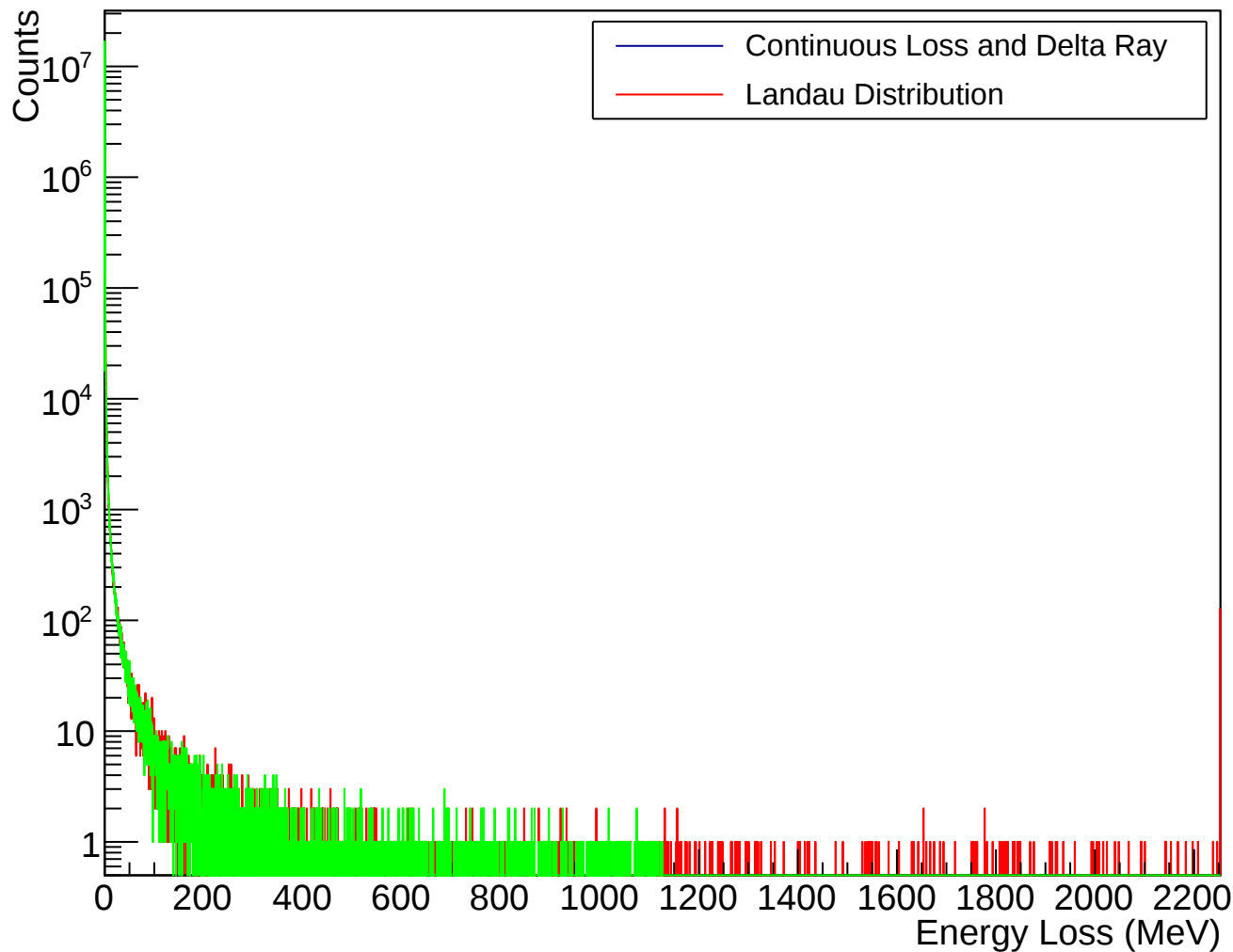
Ionization Energy Loss Distribution ( ^{12}\text{C} Thickness 1.0mm)
