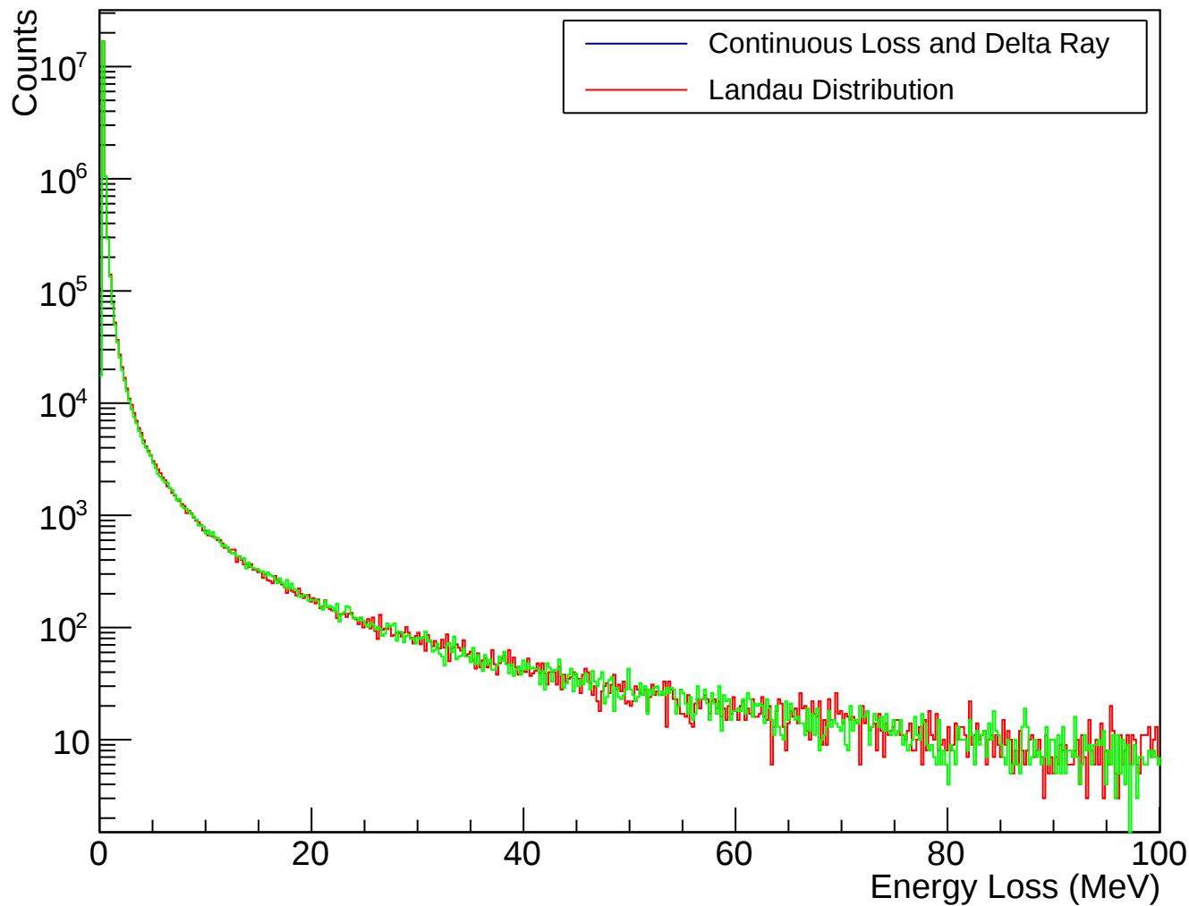
Ionization Energy Loss Distribution ( ^{12}\text{C} Thickness 1.0mm)
