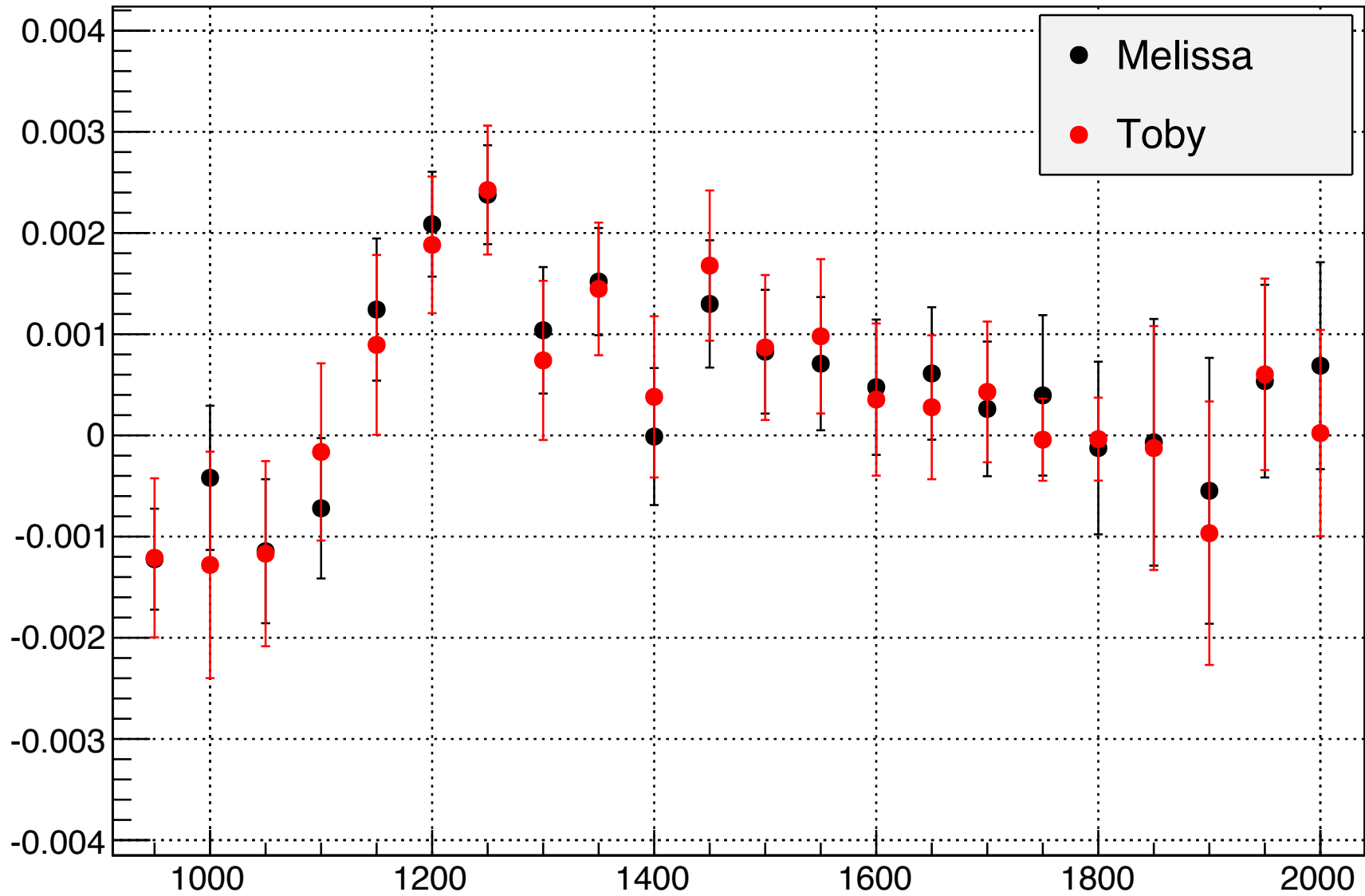
Phys Asymmetries, E = 2.2 GeV, 2.5T Target Field, Transverse
