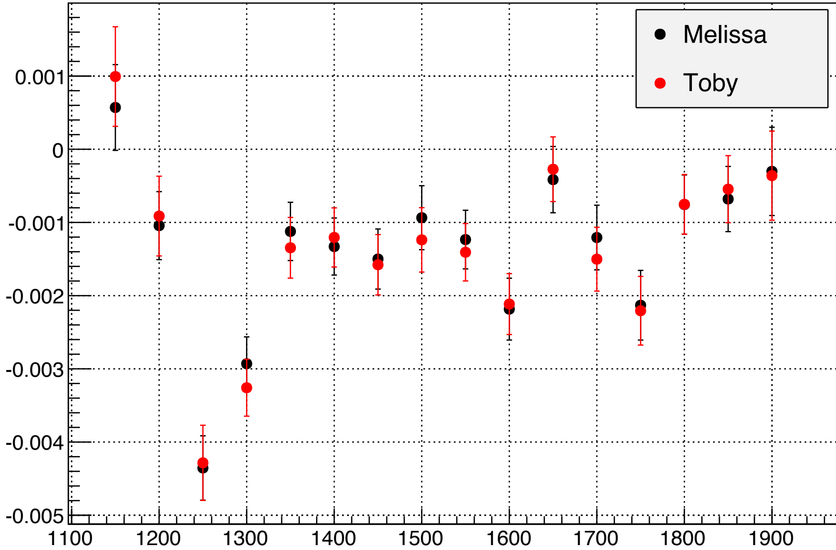
Phys Asymmetries, E = 3.3 GeV, 5T Target Field, Transverse
