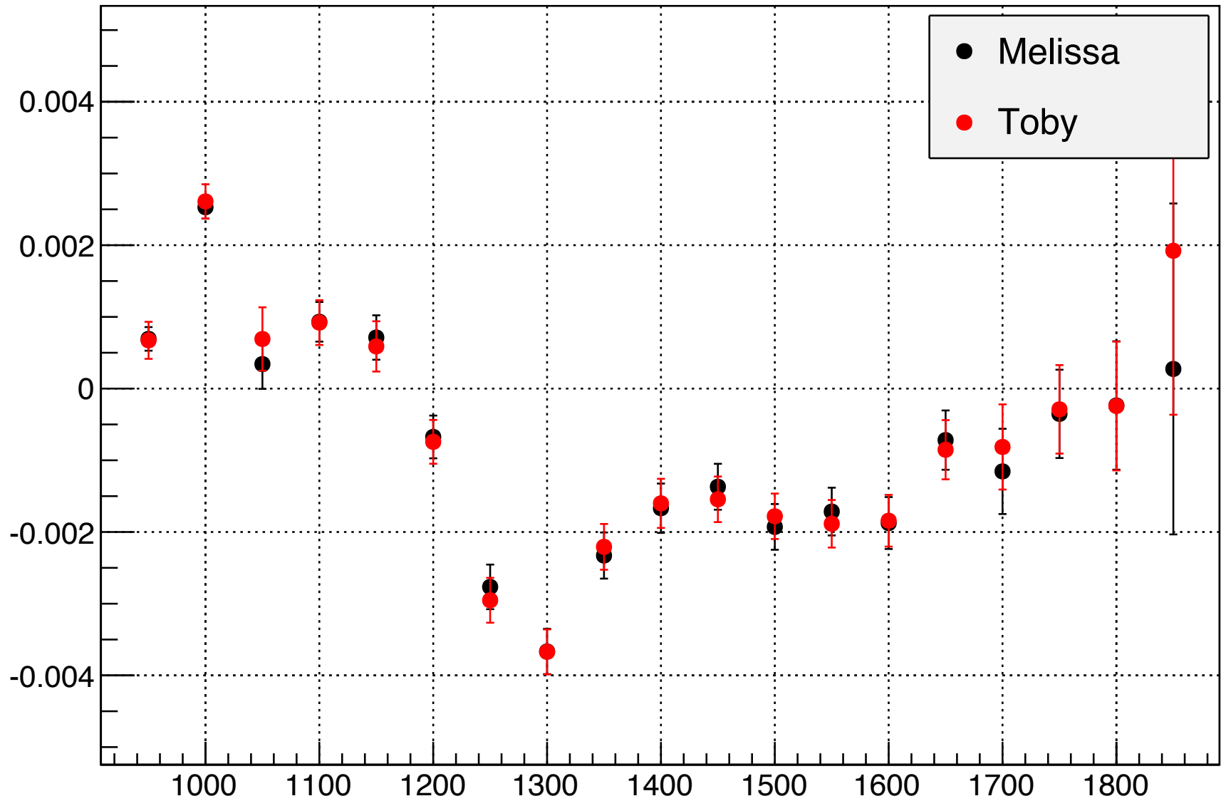
Phys Asymmetries, E = 2.2 GeV, 5T Target Field, Transverse
