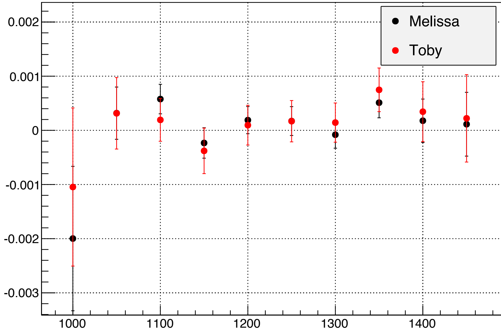
Phys Asymmetries, E = 1.1 GeV, 2.5T Target Field, Transverse
