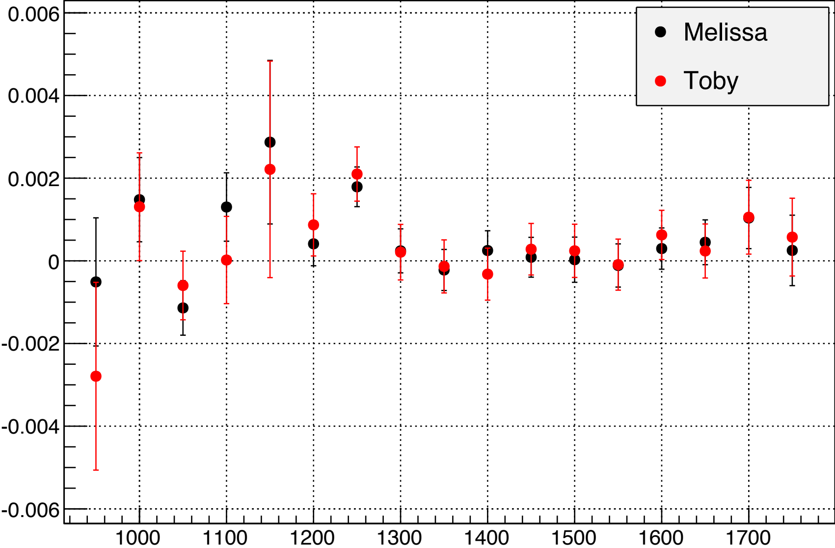
Phys Asymmetries, E = 1.7 GeV, 2.5T Target Field, Transverse
