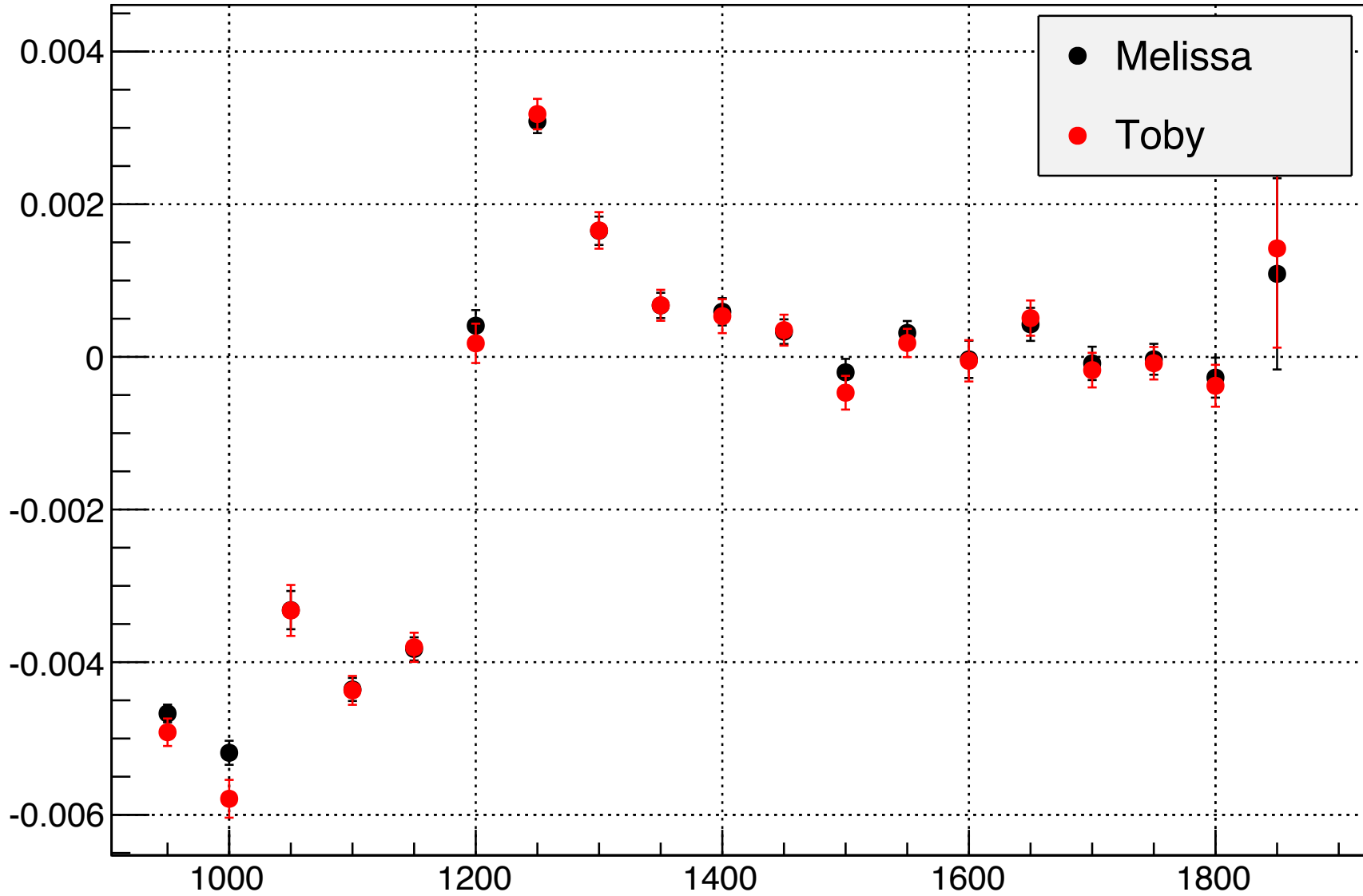
Phys Asymmetries, E = 2.2 GeV, 5T Target Field, Longitudinal
