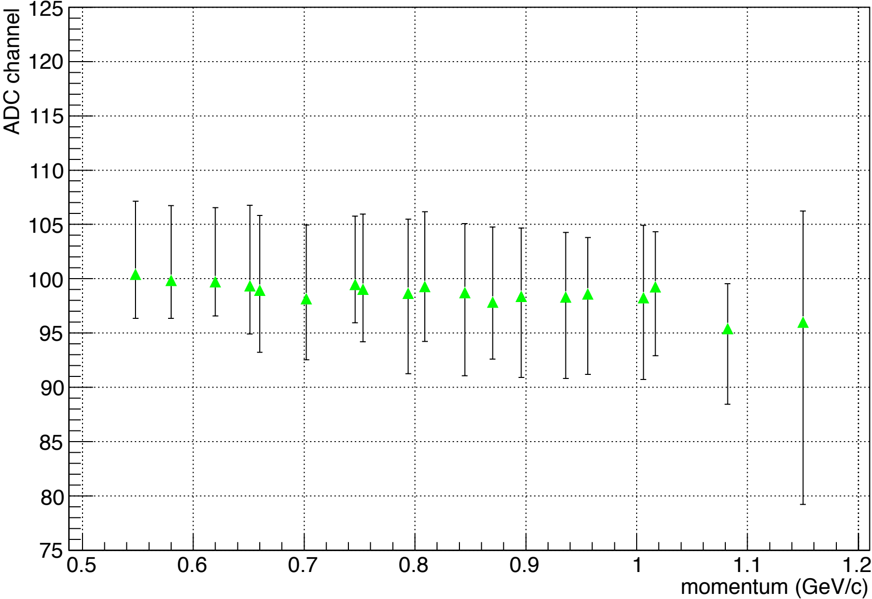
RHRS Gas Cherenkov Single Photo-electron Peak Location for 1157 MeV
