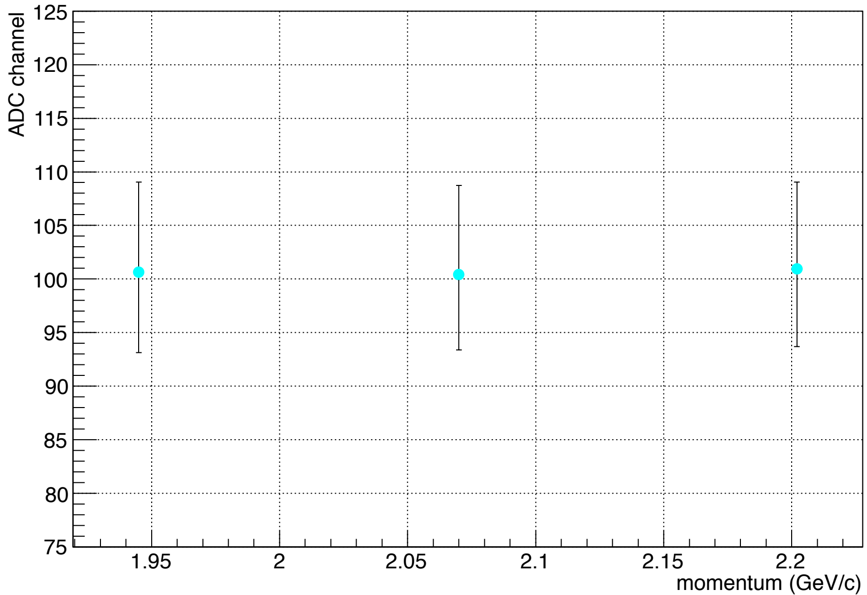
RHRS Gas Cherenkov Single Photo-electron Peak Location for 3351 MeV
