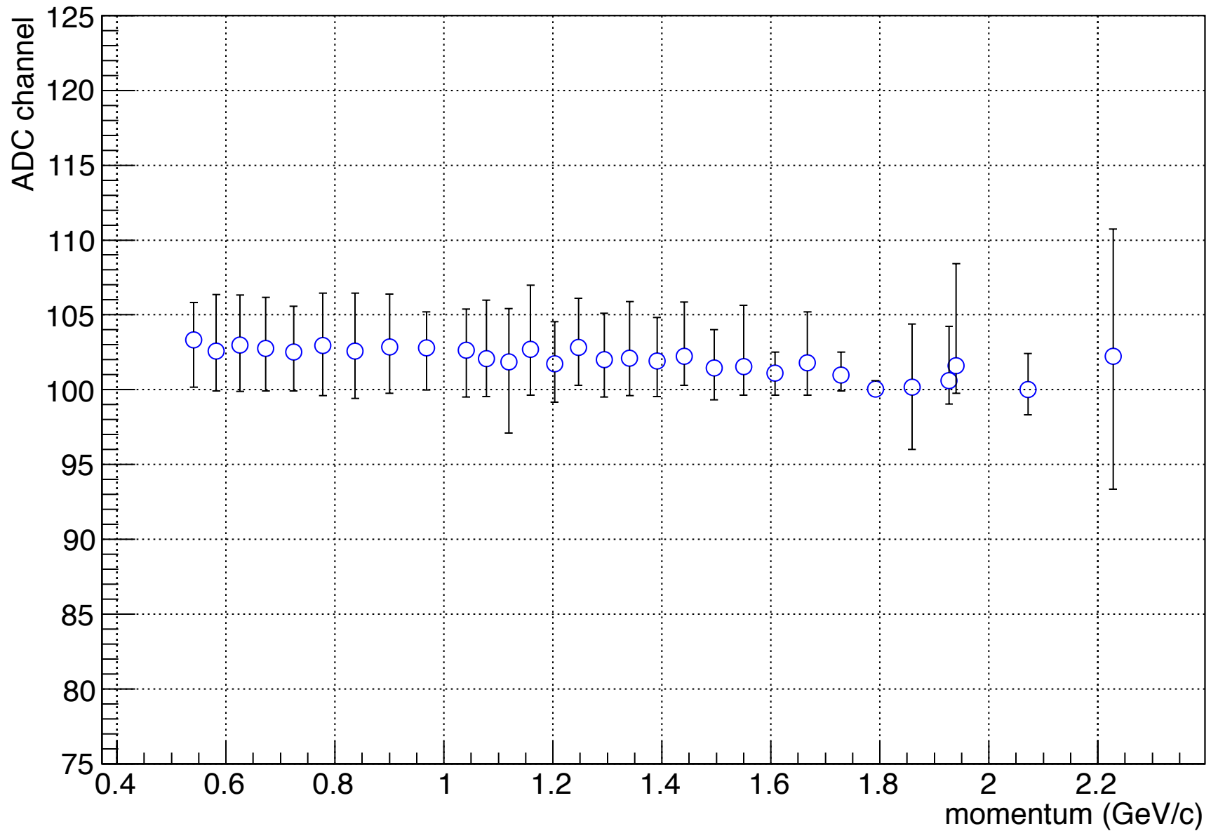
RHRS Gas Cherenkov Single Photo-electron Peak Location for 2253 MeV
