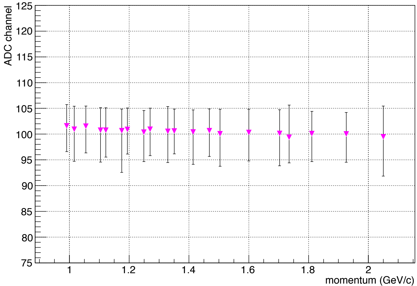
RHRS Gas Cherenkov Single Photo-electron Peak Location for 2253 (2) MeV
