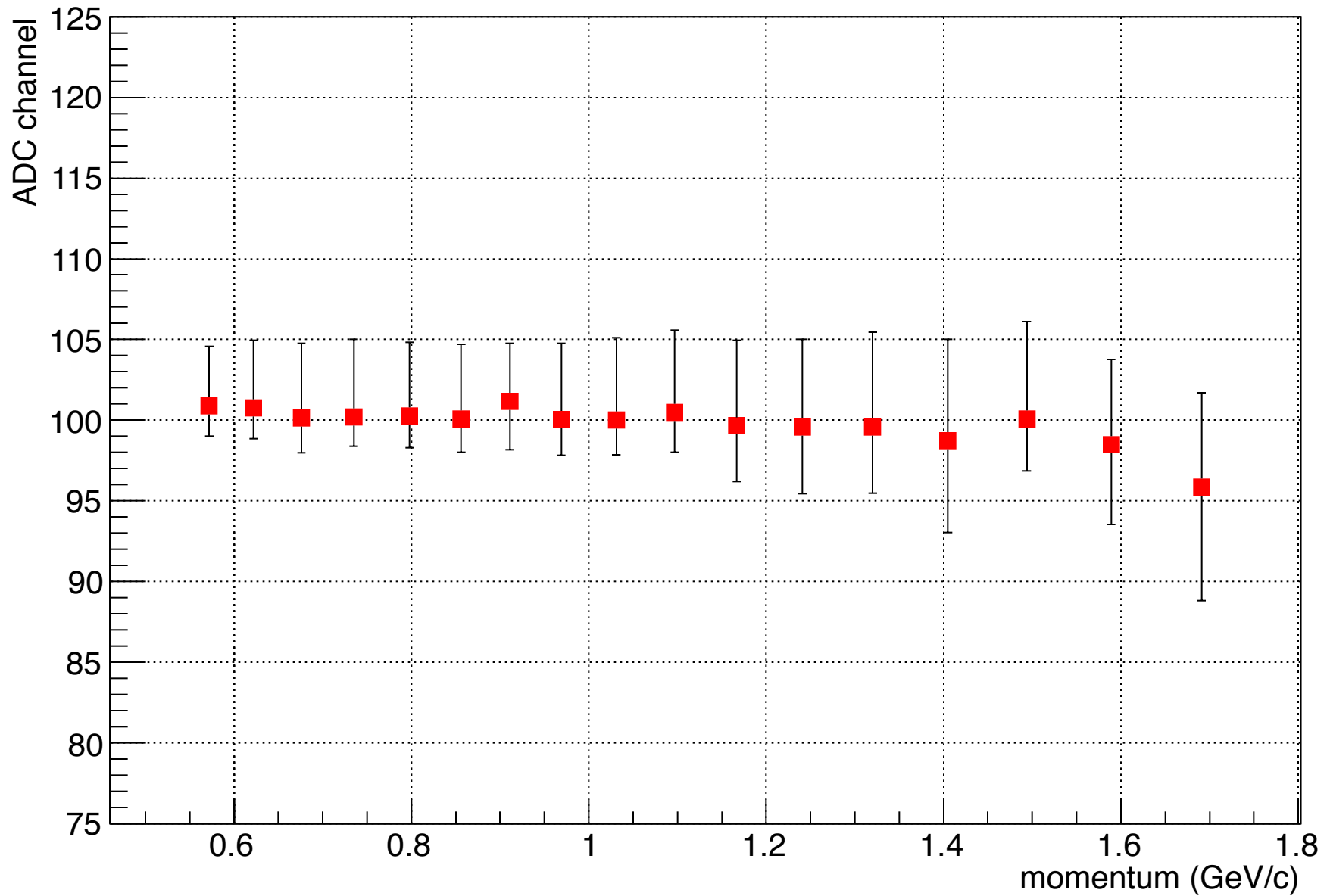
RHRS Gas Cherenkov Single Photo-electron Peak Location for 1706 MeV
