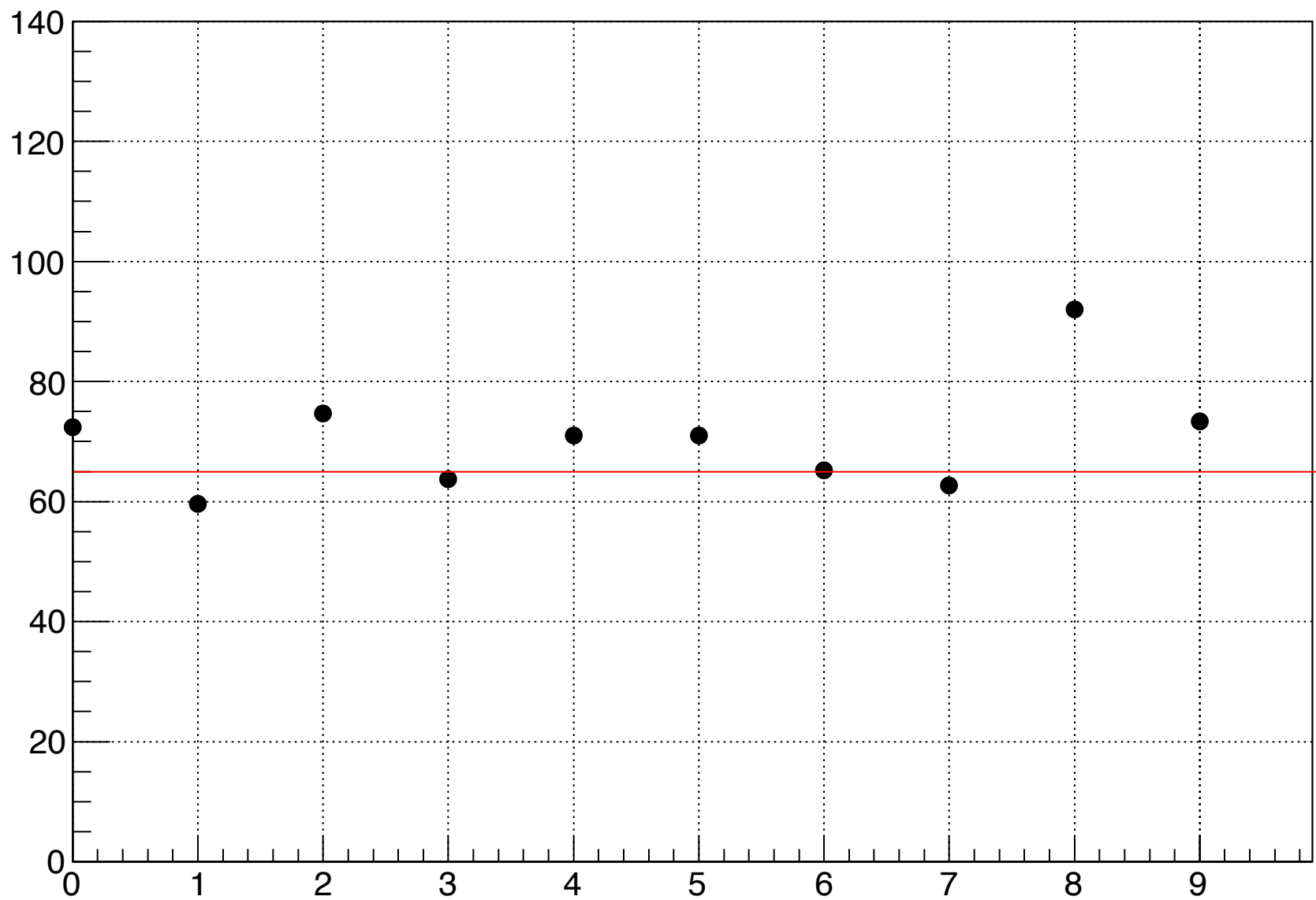
RHRS Cherenkov SPE alignment: Channel[#] vs ADC Channel
