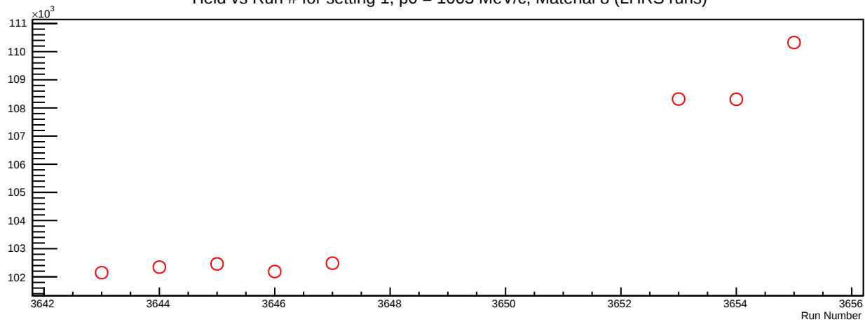
Yield vs Run # for setting 1, p0 = 1003 MeV/c, Material 8 (LHRS runs)
