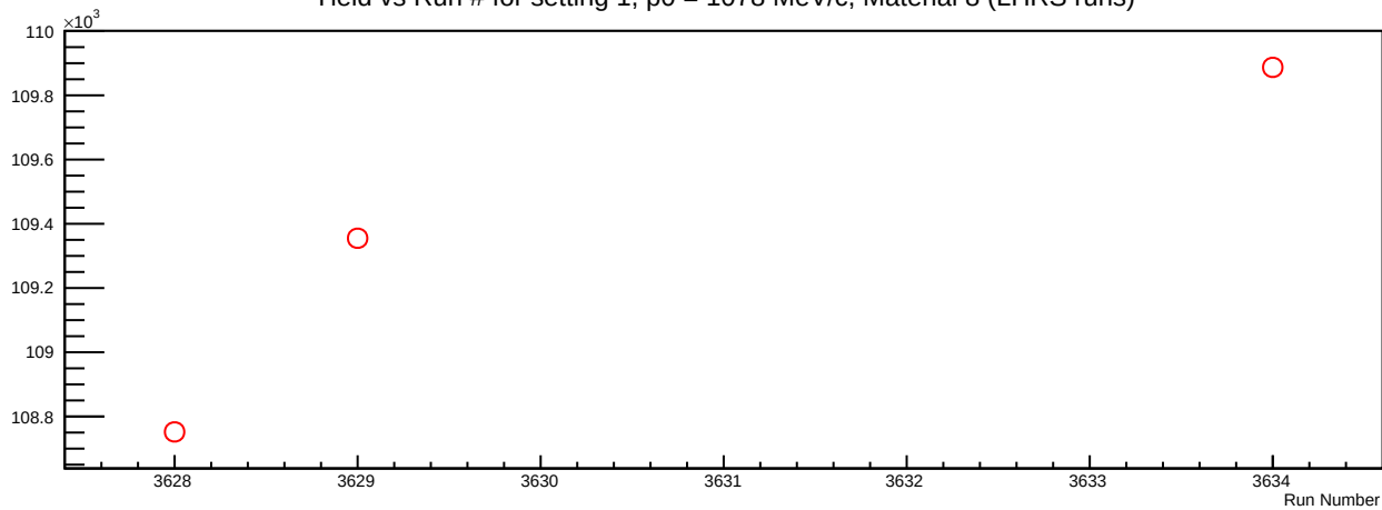
Yield vs Run # for setting 1, p_0 = 1078 MeV/c, Material 8 (LHRS runs)
