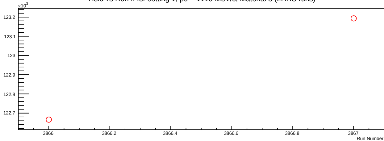
Yield vs Run # for setting 1, p_0 = 1119 MeV/c, Material 8 (LHRS runs)
