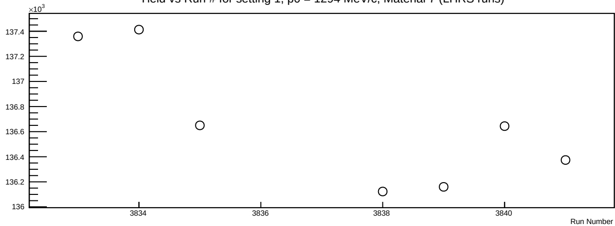
Yield vs Run # for setting 1, p0 = 1294 MeV/c, Material 7 (LHRS runs)
