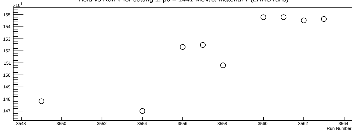
Yield vs Run # for setting 1, p0 = 1441 MeV/c, Material 7 (LHRS runs)
