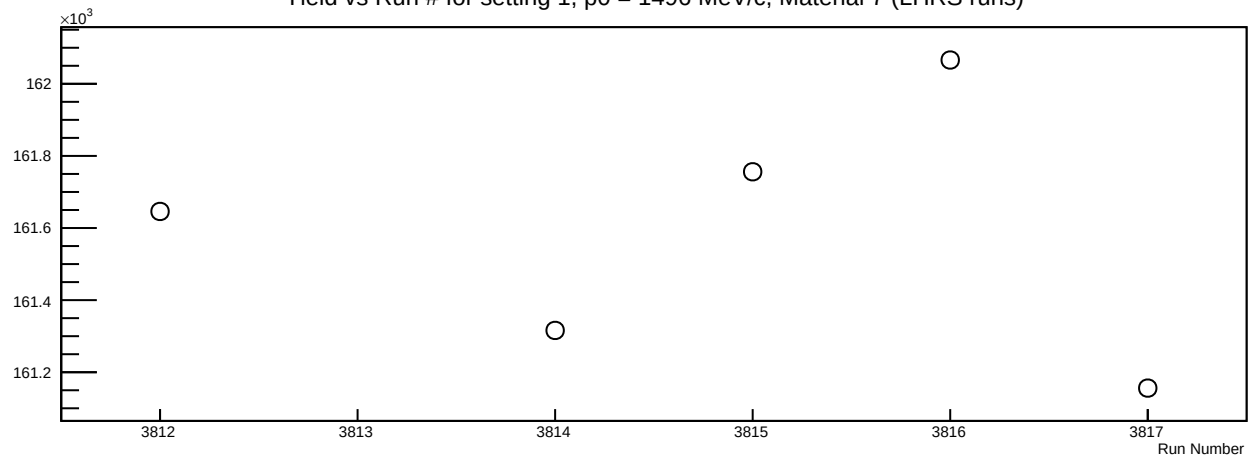
Yield vs Run # for setting 1, p0 = 1496 MeV/c, Material 7 (LHRS runs)
