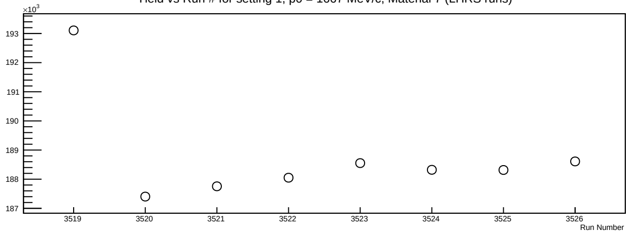
Yield vs Run # for setting 1, p0 = 1667 MeV/c, Material 7 (LHRS runs)
