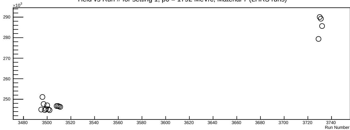
Yield vs Run # for setting 1, p_0 = 1792 MeV/c, Material 7 (LHRS runs)
