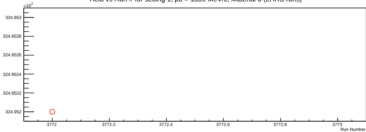
Yield vs Run # for setting 1, p0 = 1859 MeV/c, Material 8 (LHRS runs)
