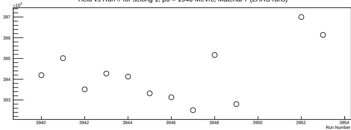
Yield vs Run # for setting 1, p0 = 1940 MeV/c, Material 7 (LHRS runs)
