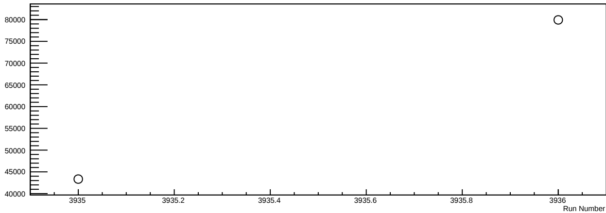
Yield vs Run # for setting 1, p_0 = 541 MeV/c, Material 7 (LHRS runs)
