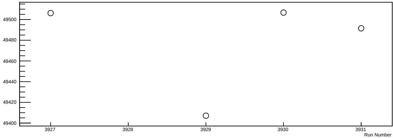
Yield vs Run # for setting 1, p_0 = 582 MeV/c, Material 7 (LHRS runs)
