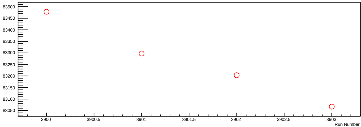
Yield vs Run # for setting 1, p_0 = 778 MeV/c, Material 8 (LHRS runs)
