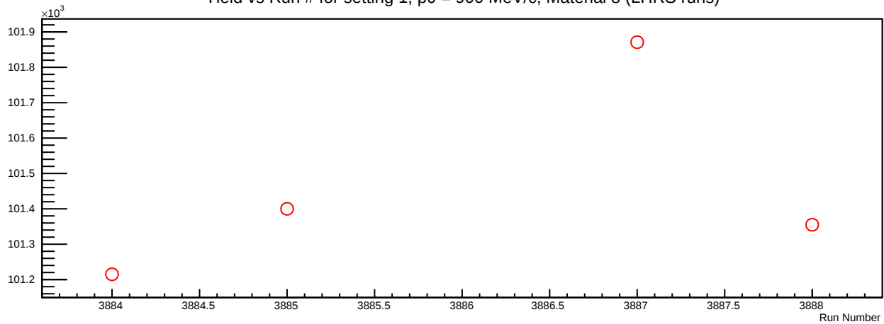
Yield vs Run # for setting 1, p_0 = 900 MeV/c, Material 8 (LHRS runs)
