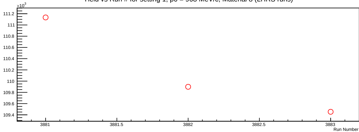
Yield vs Run # for setting 1, p_0 = 968 MeV/c, Material 8 (LHRS runs)
