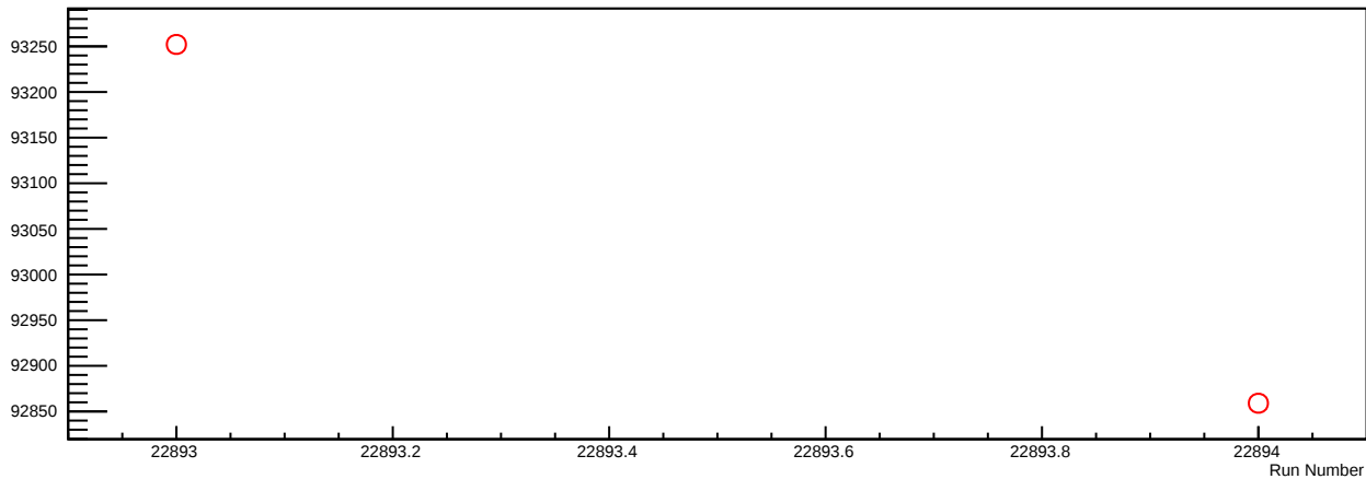
Yield vs Run # for setting 1, p_0 = 1119 MeV/c, Material 8 (RHRS runs)
