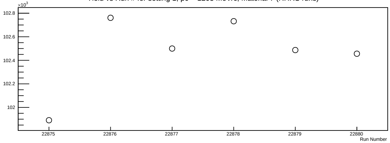
Yield vs Run # for setting 1, p_0 = 1203 MeV/c, Material 7 (RHRS runs)
