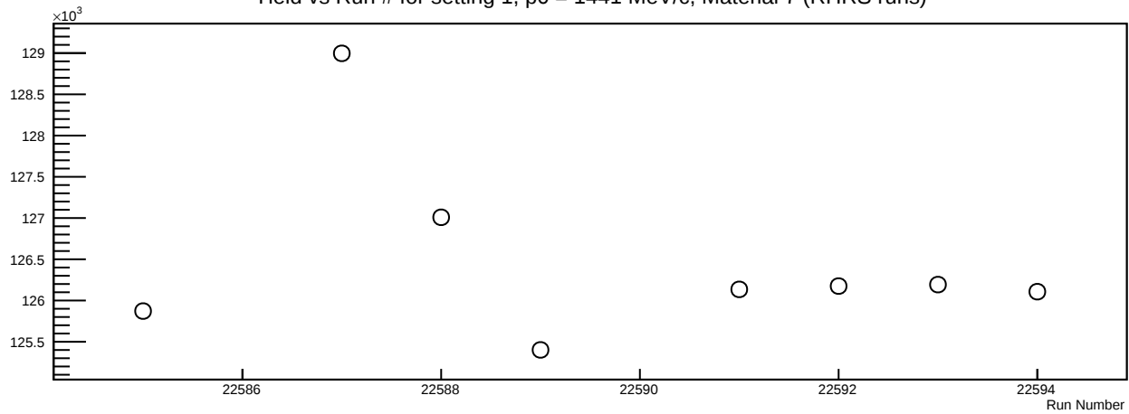
Yield vs Run # for setting 1, p0 = 1441 MeV/c, Material 7 (RHRS runs)
