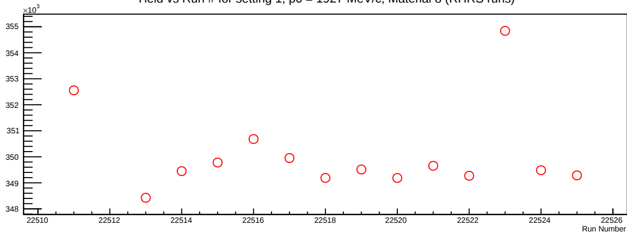
Yield vs Run # for setting 1, p_0 = 1927 MeV/c, Material 8 (RHRS runs)
