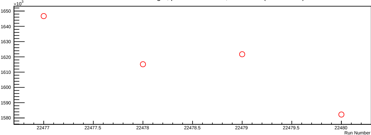
Yield vs Run # for setting 1, p0 = 2228 MeV/c, Material 8 (RHRS runs)
