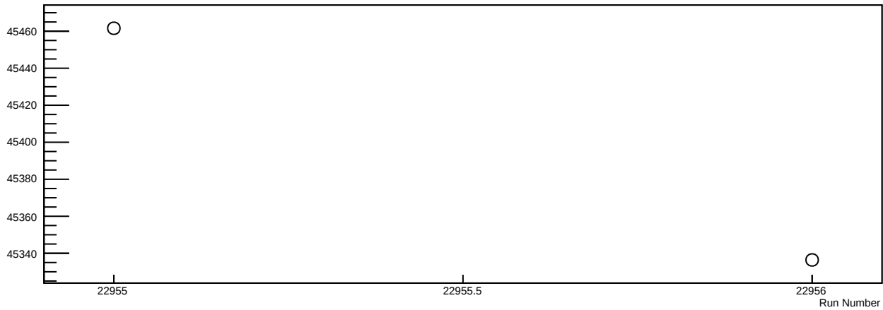
Yield vs Run # for setting 1, p_0 = 626 MeV/c, Material 7 (RHRS runs)
