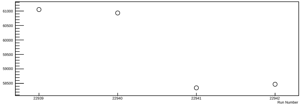
Yield vs Run # for setting 1, p_0 = 724 MeV/c, Material 7 (RHRS runs)
