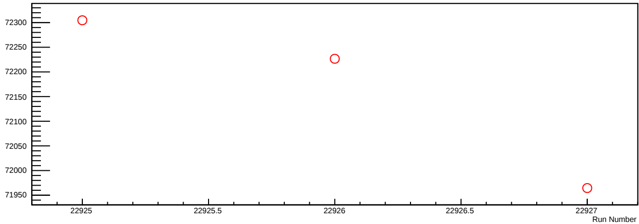
Yield vs Run # for setting 1, p_0 = 837 MeV/c, Material 8 (RHRS runs)
