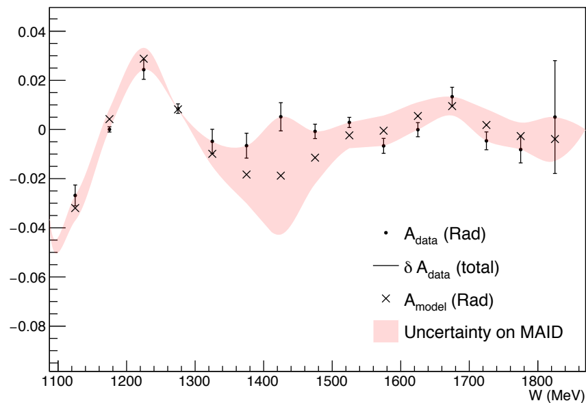
Comparison of Measured Asymmetry and Radiated Model (Longitudinal)
