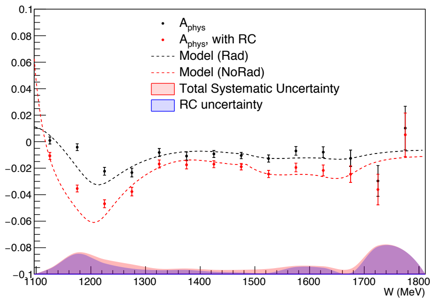
RC for Physics Asymmetries, E = 2.2 GeV, 5T Target Field, Transverse
