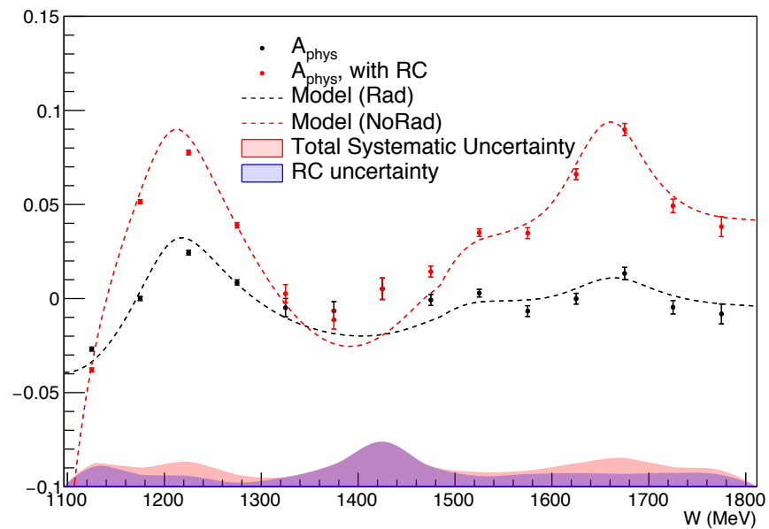
RC for Physics Asymmetries, E = 2.2 GeV, 5T Target Field, Longitudinal
