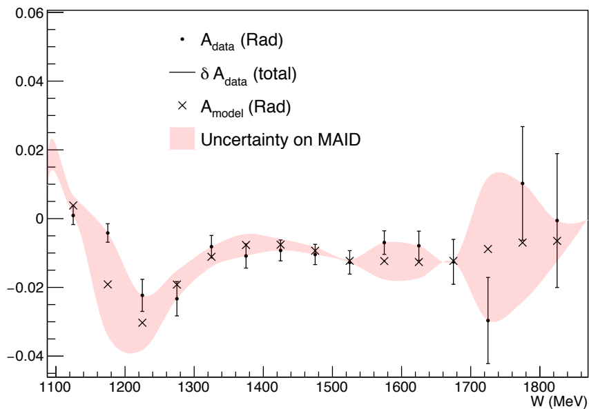
Comparison of Measured Asymmetry and Radiated Model (Transverse)
