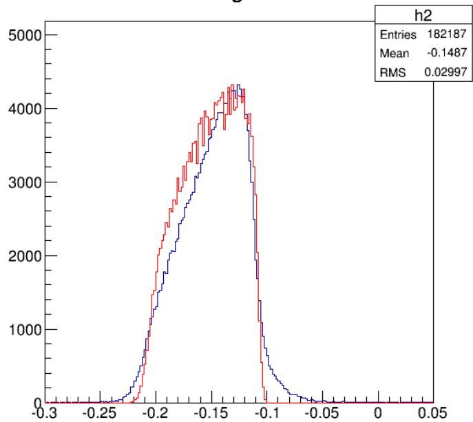
Target \theta
