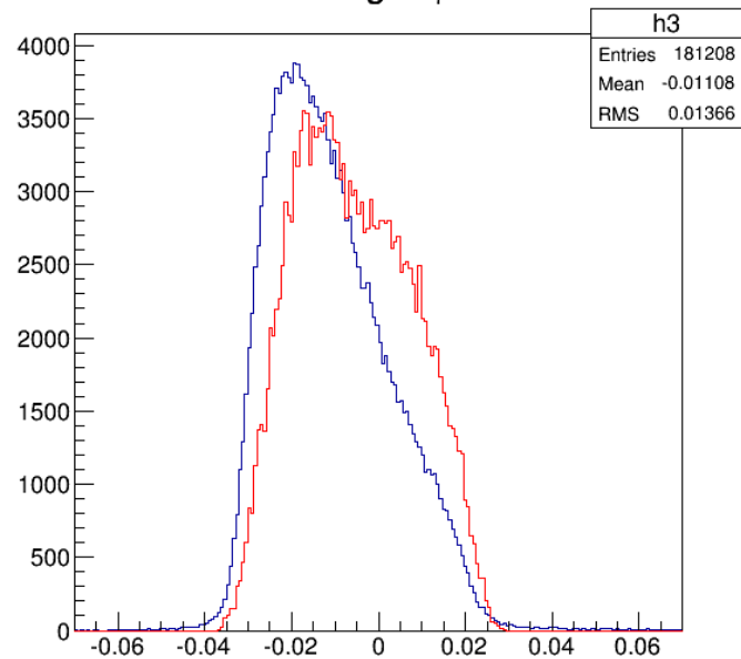
Target \phi
