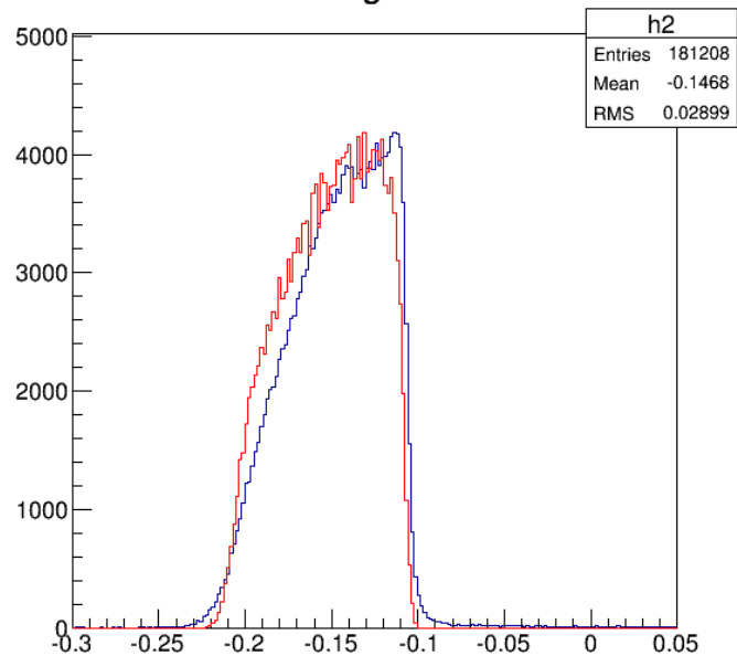
Target \theta
