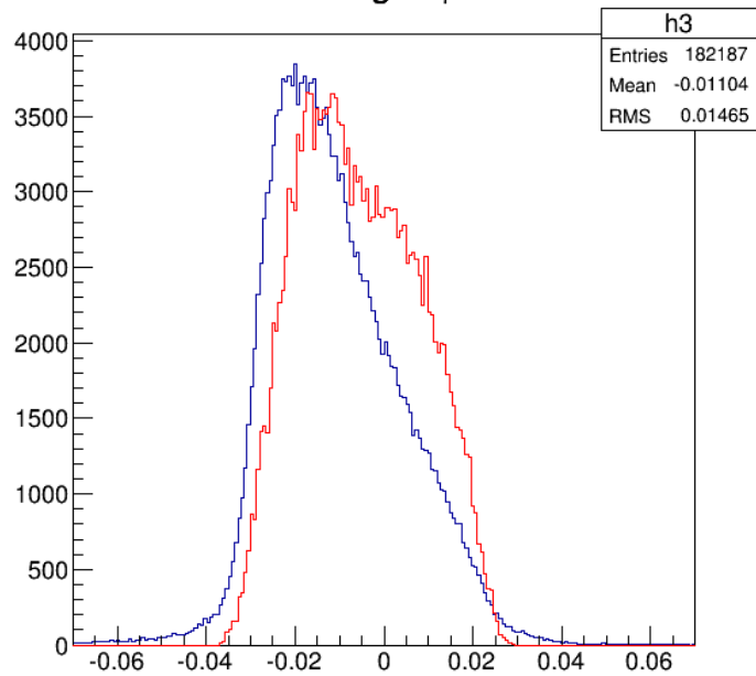
Target \phi
