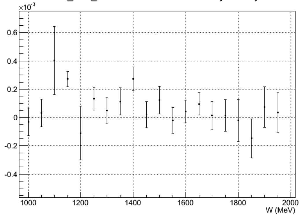
2253_25T_TRANS normalized physics asymmetry
