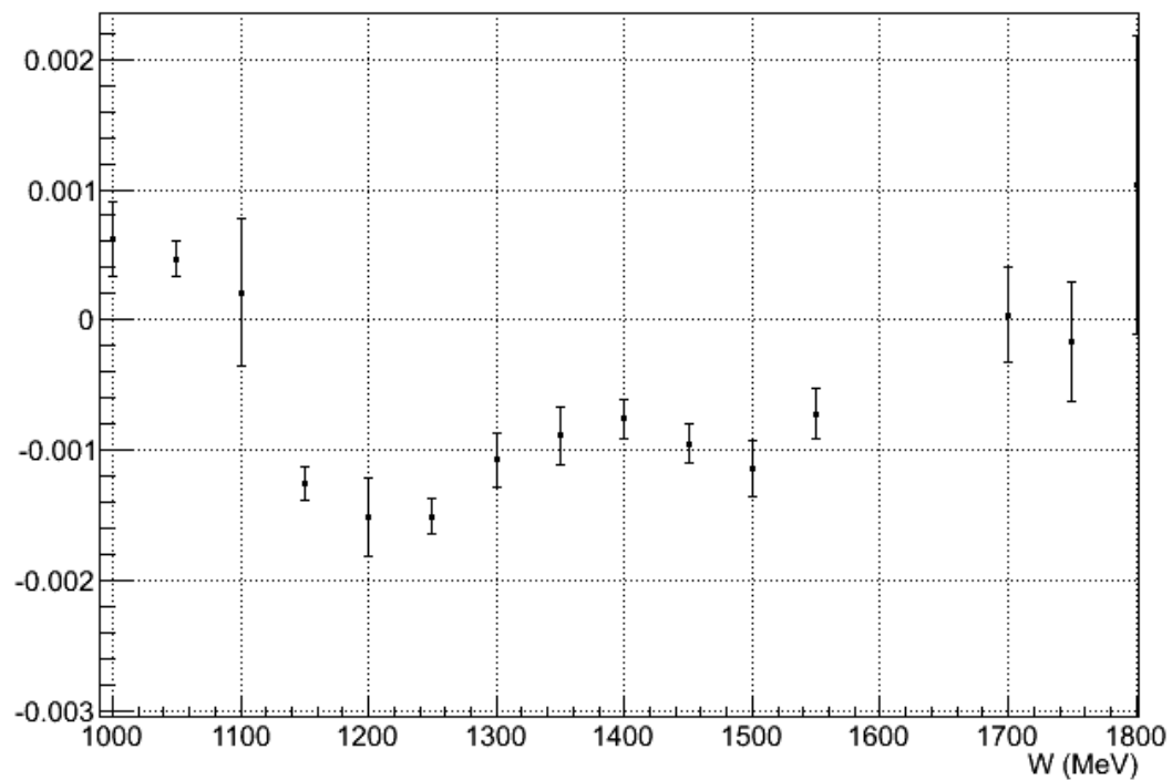
2253_5T_TRANS normalized physics asymmetry
