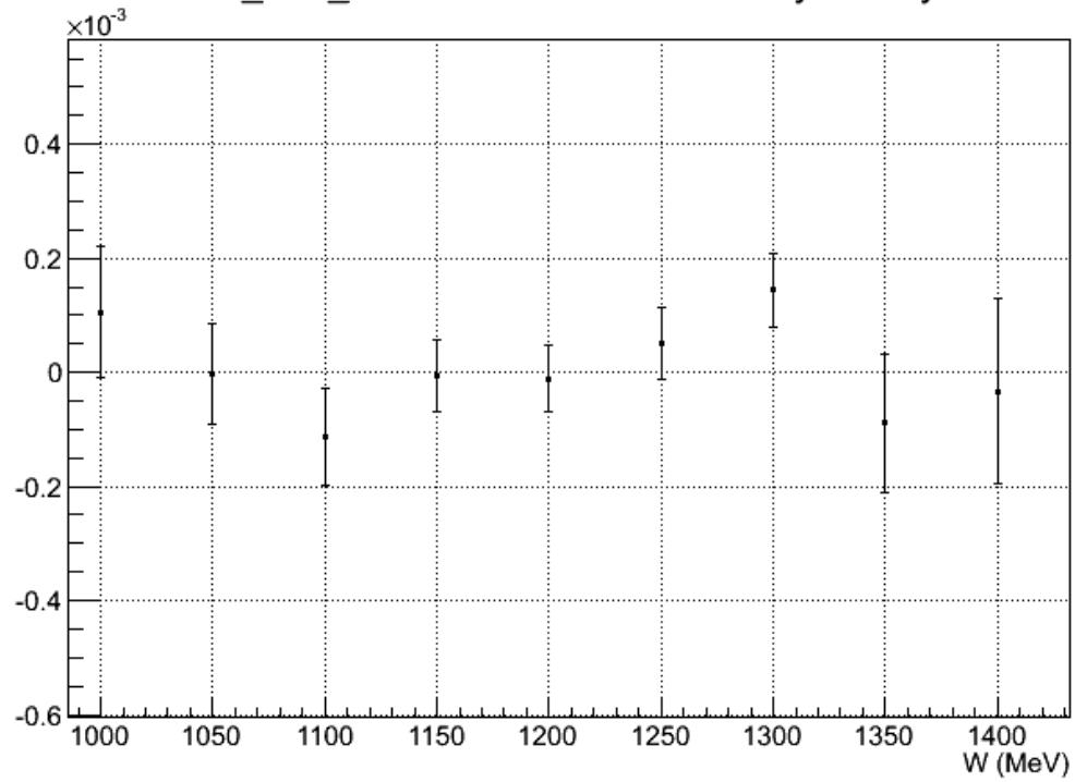
1157_25T_TRANS normalized physics asymmetry
