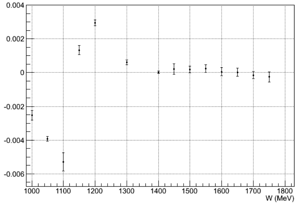
2253_5T_LONG normalized physics asymmetry
