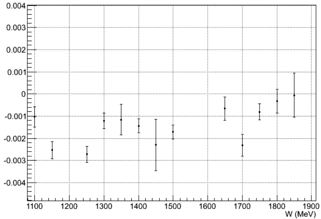
3351_5T_TRANS normalized physics asymmetry
