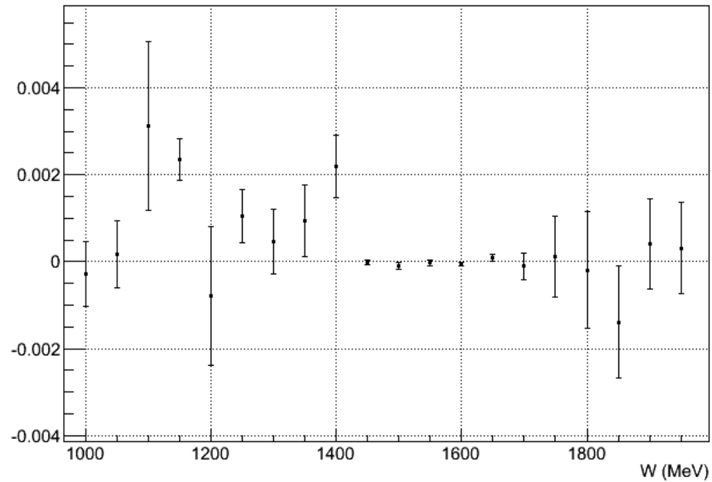
2253_25T_TRANS normalized physics asymmetry
