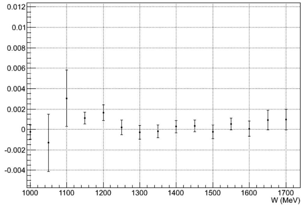
1710_25T_TRANS normalized physics asymmetry
