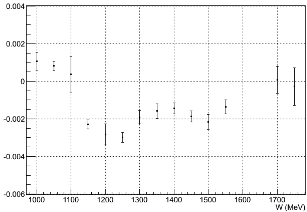
2253_5T_TRANS normalized physics asymmetry
