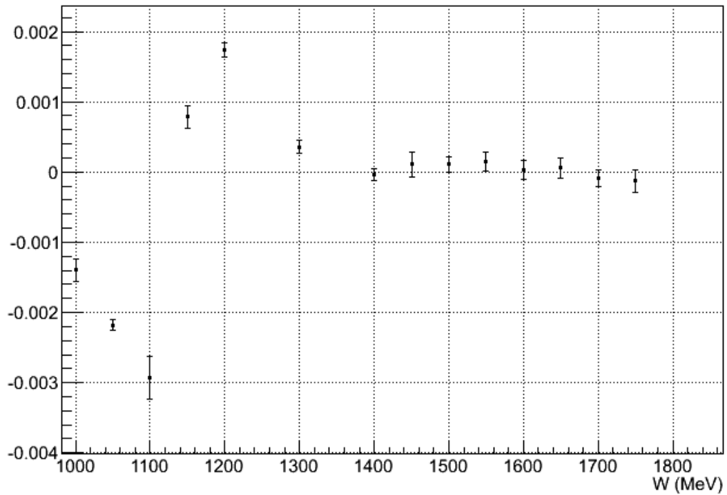
2253_5T_LONG normalized physics asymmetry
