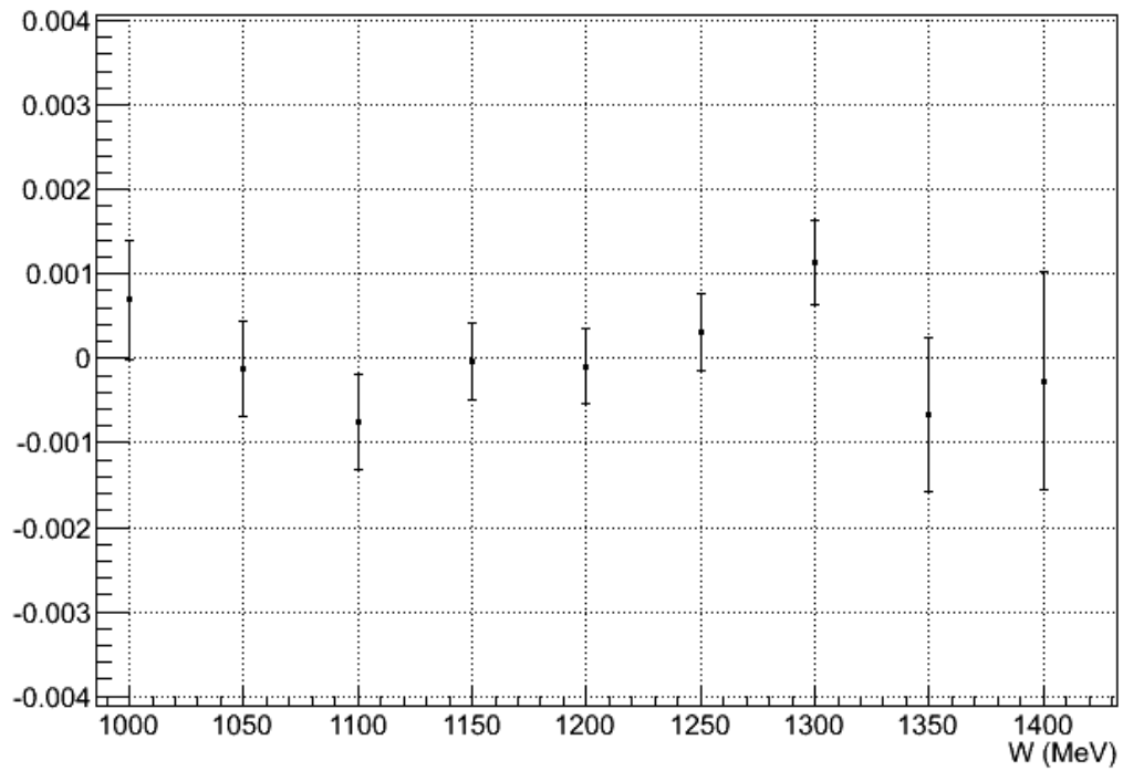
1157_25T_TRANS normalized physics asymmetry
