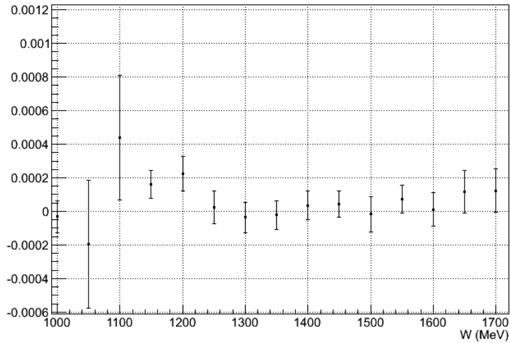
1710_25T_TRANS normalized physics asymmetry
