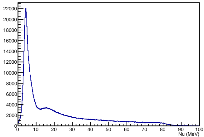
1.710GeV 2.5T Transverse
