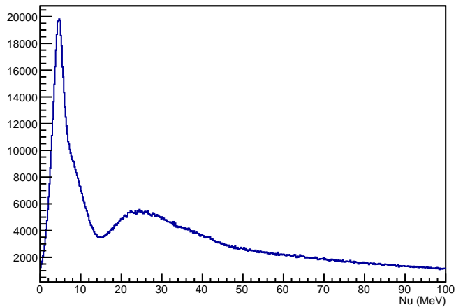
1.157GeV 2.5T Transverse
