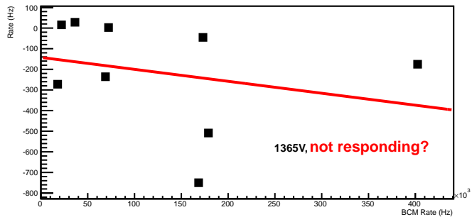
Lumi8 ped subtracted rate vs BCM
