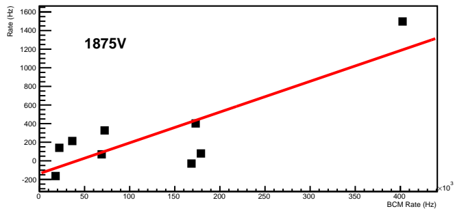
Lumi6 ped subtracted rate vs BCM
