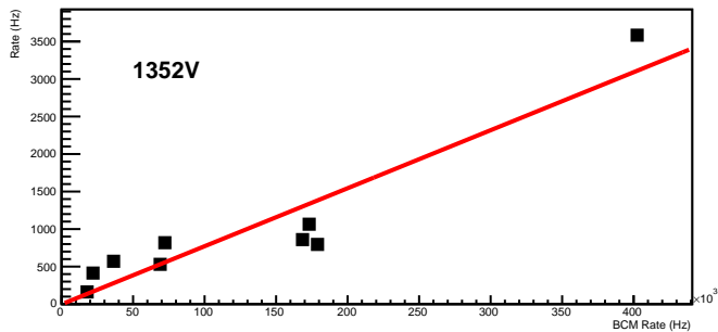
Lumi7 ped subtracted rate vs BCM
