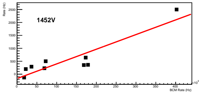
Lumi1 ped subtracted rate vs BCM
