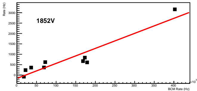
Lumi5 ped subtracted rate vs BCM
