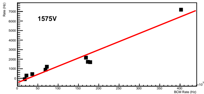
Lumi3 ped subtracted rate vs BCM
