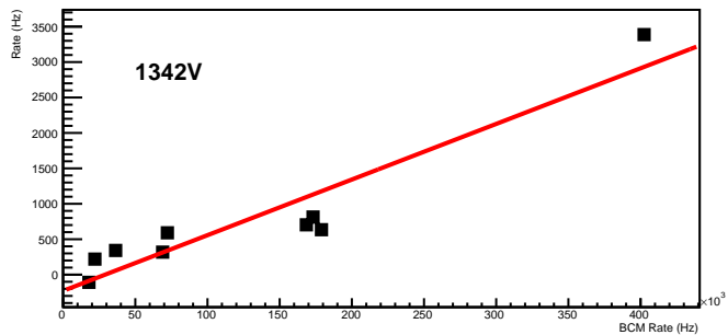
Lumi2 ped subtracted rate vs BCM
