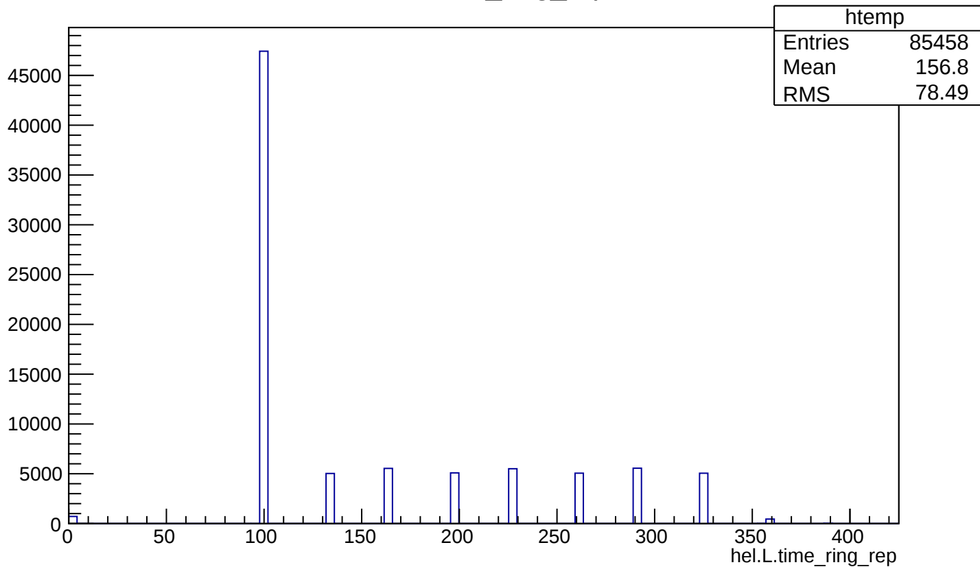
hel.L.time_ring_rep
