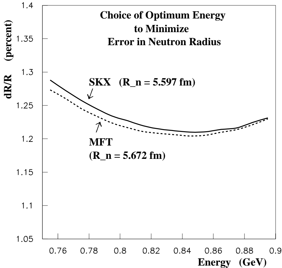
FIG. 4. Error in the neutron radius in Pb versus beam energy, for two models of the neutron radius, SKX [18] and MFT [31]. This shows that the optimum choice of energy for a measurement is not very sensitive to the value of R_n , and also provides an indication of the insensitivity to the model.
