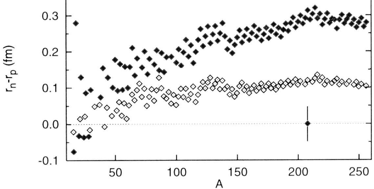
FIG. 1. The difference between neutron radii R_n = r_n and proton radii R_p = r_p for several nuclei of different mass number A . The filled symbols are for the relativistic mean field NL1 interaction while the open symbols are for the nonrelativistic zero range Skyrme skiii interaction. This figure is taken from calculations of Ring et.al [14]. A possible 1% measurement in ^{208}\text{Pb} is indicated by the error bar which has been arbitrarily placed at R_n - R_p = 0 .
