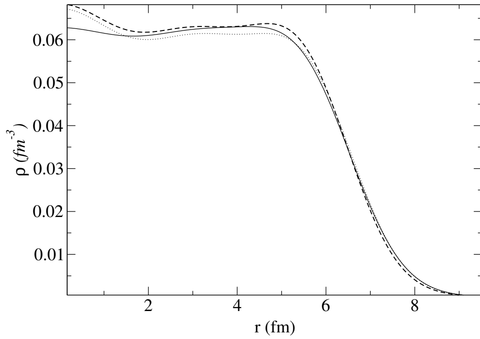
FIG. 6. The charge density in ^{208}\text{Pb} . The dotted curve is a mean field calculation with a reasonable surface energy [30] while the thick dashed curve is a mean field calculation with a very high surface energy [31]. The experimental charge density is the solid curve.
