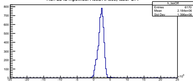
Run 2542 mpwise: Acc0/NAcc0, laser OFF
