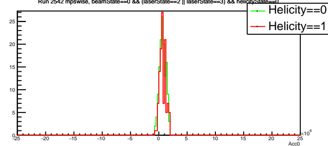
Run 2542 mpwise, beamState==0 &amp;&amp; (laserState==2 || laserState==3) &amp;&amp; helicityState==0
