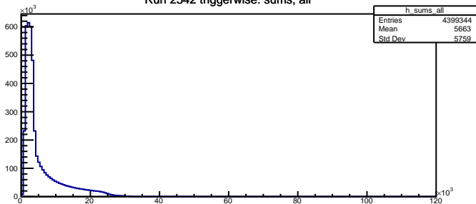
Run 2542 triggerwise: sums, all
