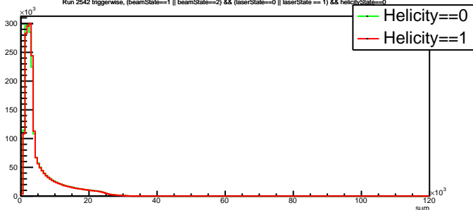
Run 2542 triggerwise, (beamState==1 || beamState==2) &amp;&amp; (laserState==0 || laserState == 1) &amp;&amp; helicityState==0
