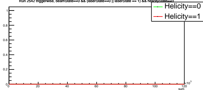
Run 2542 triggerwise, beamState==0 &amp;&amp; (laserState==0 || laserState == 1) &amp;&amp; helicityState==0
