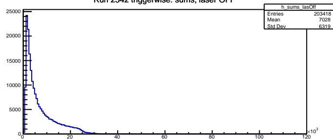
Run 2542 triggerwise: sums, laser OFF
