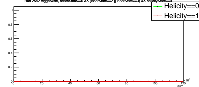
Run 2542 triggerwise, beamState==0 &amp;&amp; (laserState==2 || laserState==3) &amp;&amp; helicityState==0
