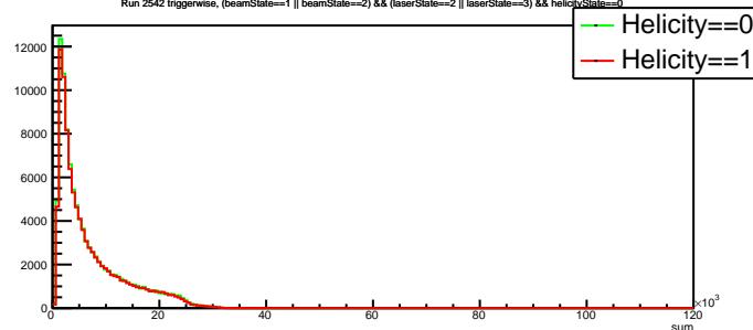
Run 2542 triggerwise, (beamState==1 || beamState==2) &amp;&amp; (laserState==2 || laserState==3) &amp;&amp; helicityState==0
