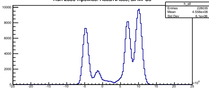
Run 2650 mpwise: Acc0/NAcc0, all MPSs
