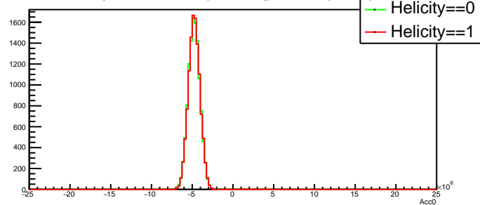
Run 2650 mpwise, beamState==0 &amp;&amp; (laserState==0 || laserState == 1) &amp;&amp; helicityState==0
