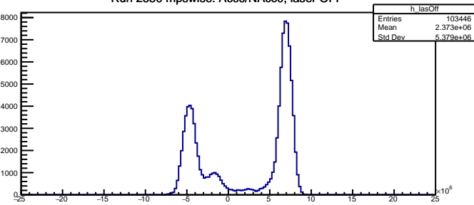
Run 2650 mpwise: Acc0/NAcc0, laser OFF
